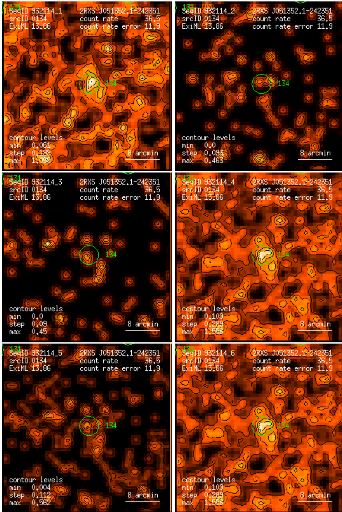
Figure 134: RASS 932114: detection 0134: band rate images, Gaussian filter: (1) PSPC channels 11 – 41, (2) 52 – 90, (3) 91 – 201, (4) 11 – 235, (5) 52 – 201, (6) 11 – 201. Broad band rates in counts/ks. Band rate contour levels in counts/ks/arcmin 2 .
