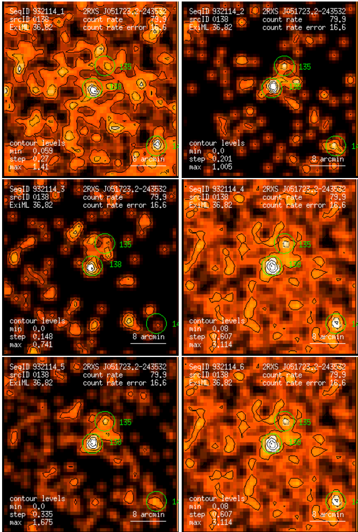
Figure 138: RASS 932114: detection 0138: band rate images, Gaussian filter: (1) PSPC channels 11 – 41, (2) 52 – 90, (3) 91 – 201, (4) 11 – 235, (5) 52 – 201, (6) 11 – 201. Broad band rates in counts/ks. Band rate contour levels in counts/ks/arcmin 2 .
