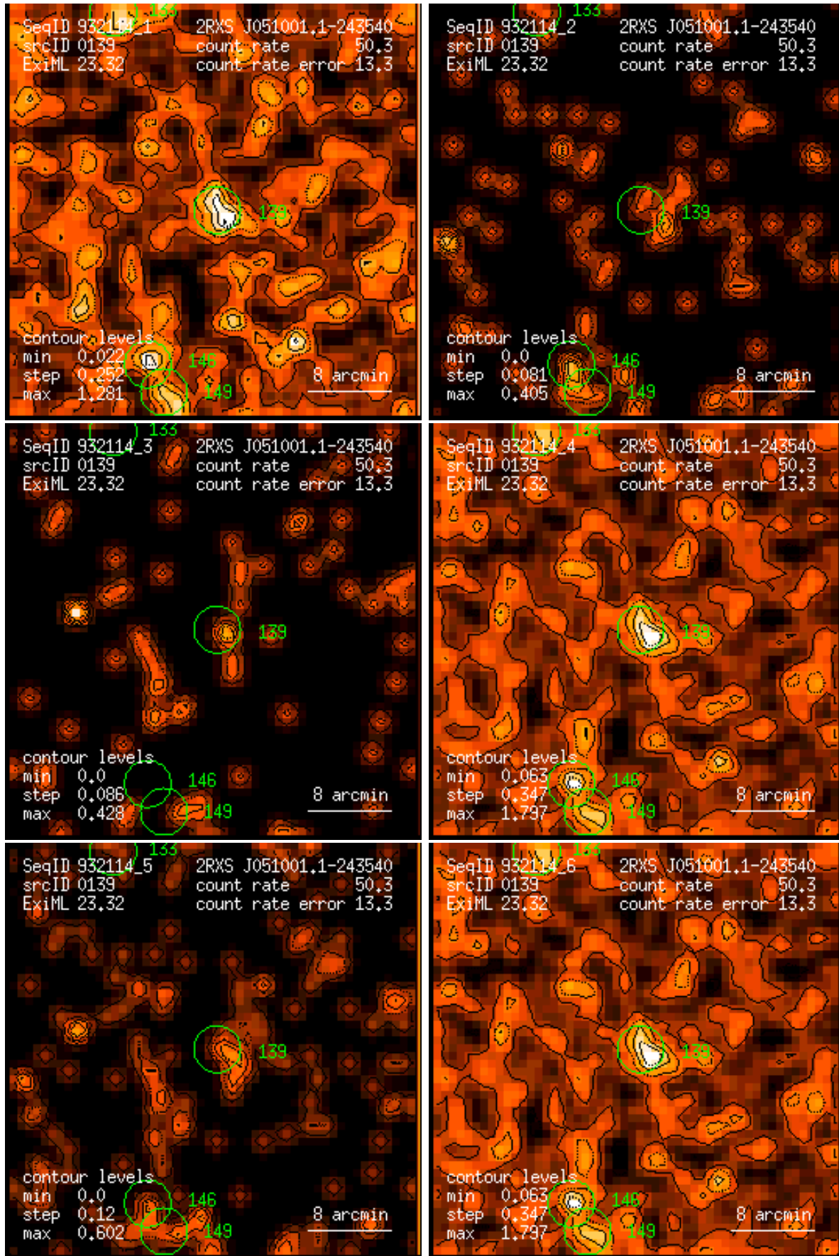
Figure 139: RASS 932114: detection 0139: band rate images, Gaussian filter: (1) PSPC channels 11 – 41, (2) 52 – 90, (3) 91 – 201, (4) 11 – 235, (5) 52 – 201, (6) 11 – 201. Broad band rates in counts/ks. Band rate contour levels in counts/ks/arcmin 2 .
