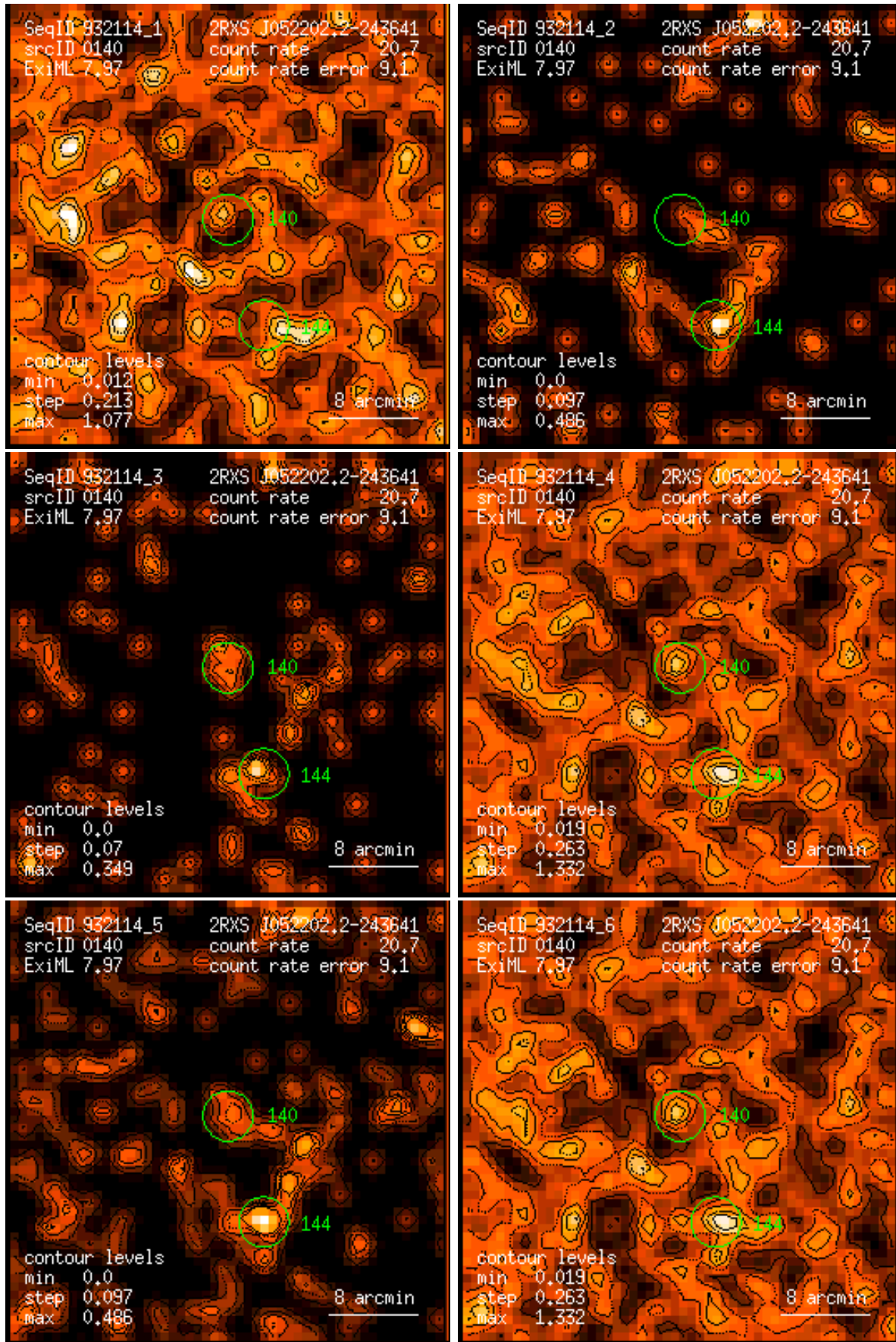
Figure 140: RASS 932114: detection 0140: band rate images, Gaussian filter: (1) PSPC channels 11 – 41, (2) 52 – 90, (3) 91 – 201, (4) 11 – 235, (5) 52 – 201, (6) 11 – 201. Broad band rates in counts/ks. Band rate contour levels in counts/ks/arcmin 2 .
