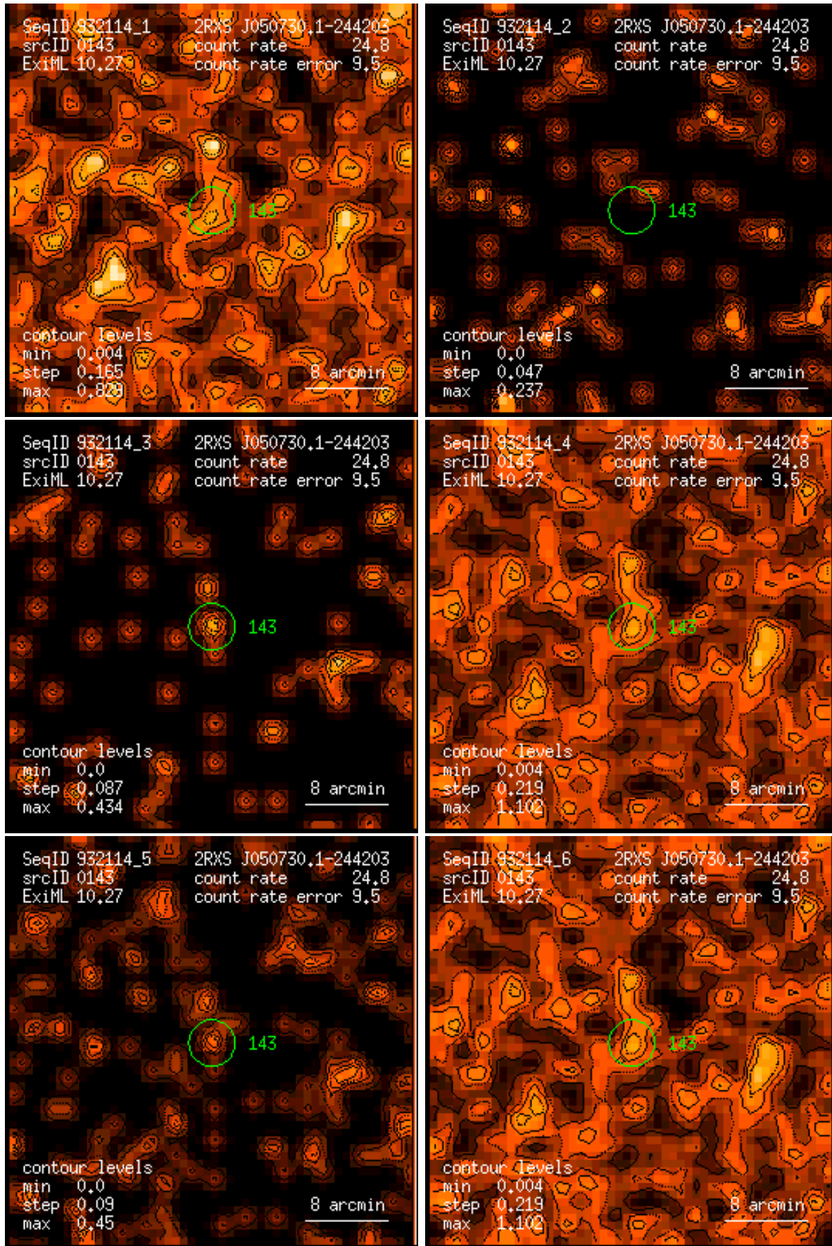
Figure 143: RASS 932114: detection 0143: band rate images, Gaussian filter: (1) PSPC channels 11 – 41, (2) 52 – 90, (3) 91 – 201, (4) 11 – 235, (5) 52 – 201, (6) 11 – 201. Broad band rates in counts/ks. Band rate contour levels in counts/ks/arcmin 2 .
