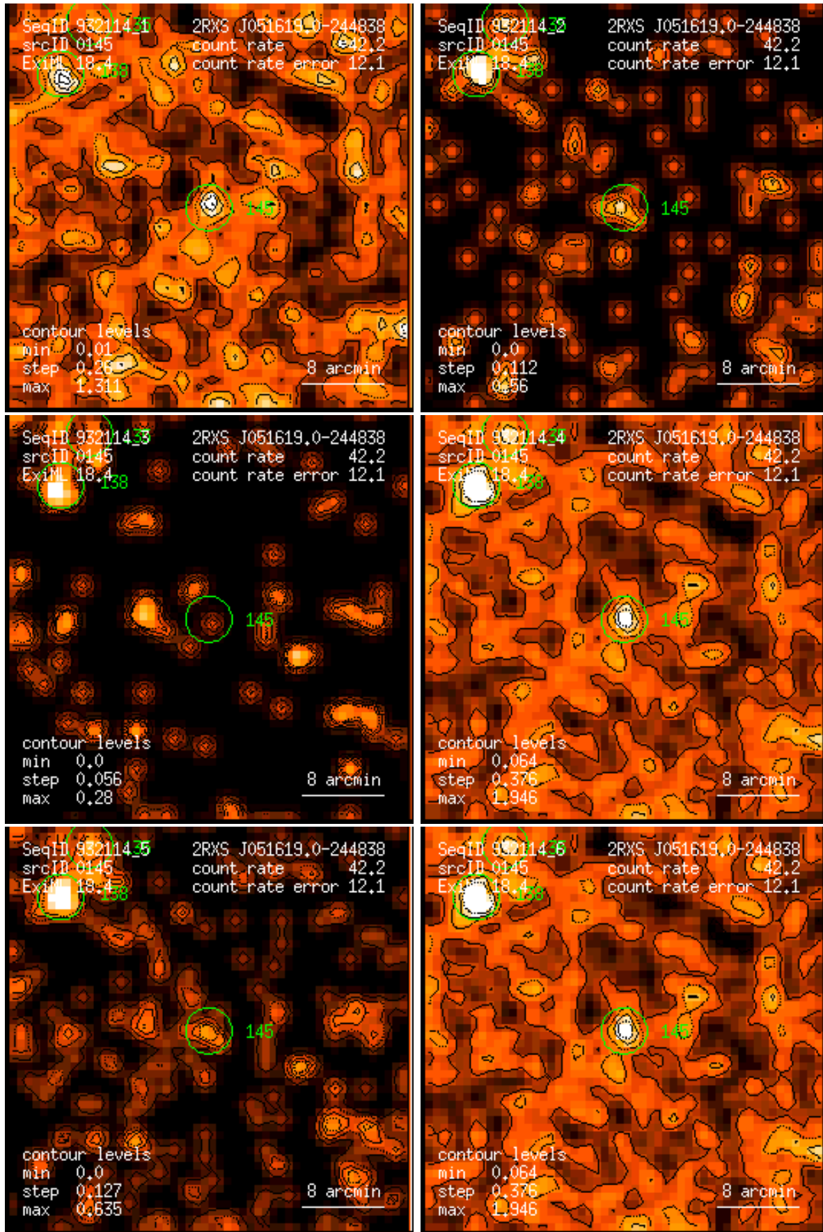
Figure 145: RASS 932114: detection 0145: band rate images, Gaussian filter: (1) PSPC channels 11 – 41, (2) 52 – 90, (3) 91 – 201, (4) 11 – 235, (5) 52 – 201, (6) 11 – 201. Broad band rates in counts/ks. Band rate contour levels in counts/ks/arcmin 2 .
