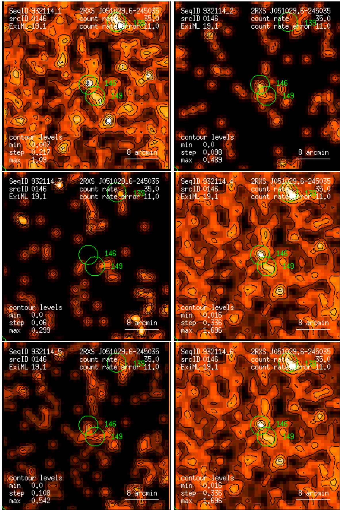
Figure 146: RASS 932114: detection 0146: band rate images, Gaussian filter: (1) PSPC channels 11 – 41, (2) 52 – 90, (3) 91 – 201, (4) 11 – 235, (5) 52 – 201, (6) 11 – 201. Broad band rates in counts/ks. Band rate contour levels in counts/ks/arcmin 2 .
