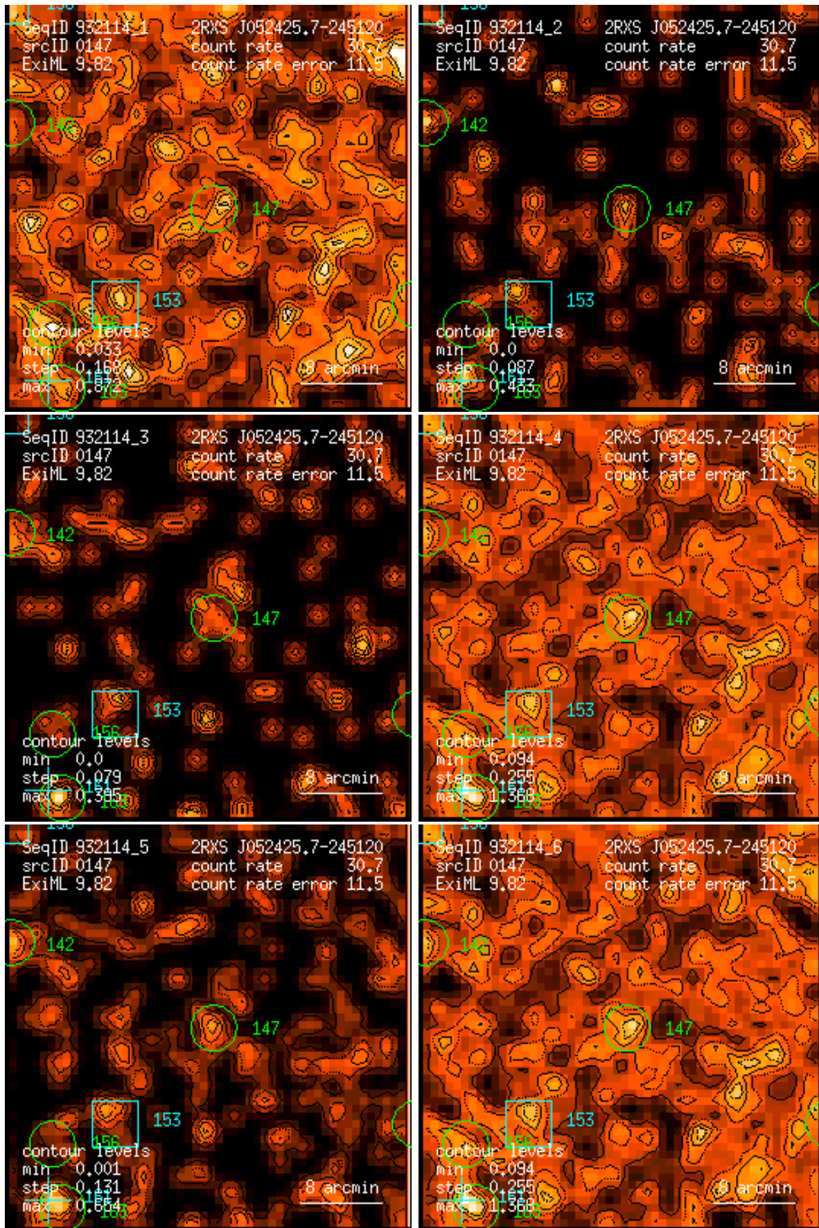
Figure 147: RASS 932114: detection 0147: band rate images, Gaussian filter: (1) PSPC channels 11 – 41, (2) 52 – 90, (3) 91 – 201, (4) 11 – 235, (5) 52 – 201, (6) 11 – 201. Broad band rates in counts/ks. Band rate contour levels in counts/ks/arcmin 2 .
