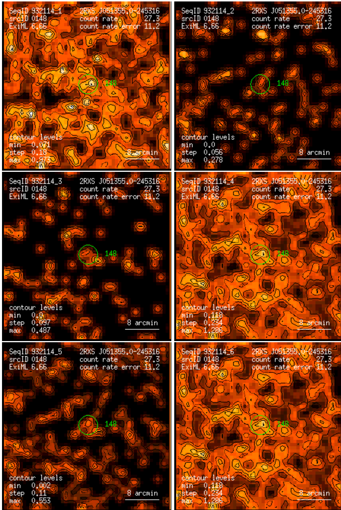
Figure 148: RASS 932114: detection 0148: band rate images, Gaussian filter: (1) PSPC channels 11 – 41, (2) 52 – 90, (3) 91 – 201, (4) 11 – 235, (5) 52 – 201, (6) 11 – 201. Broad band rates in counts/ks. Band rate contour levels in counts/ks/arcmin 2 .
