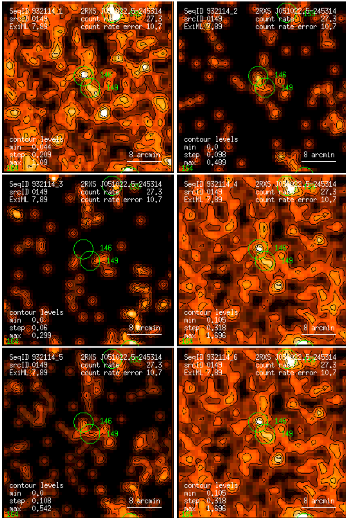
Figure 149: RASS 932114: detection 0149: band rate images, Gaussian filter: (1) PSPC channels 11 – 41, (2) 52 – 90, (3) 91 – 201, (4) 11 – 235, (5) 52 – 201, (6) 11 – 201. Broad band rates in counts/ks. Band rate contour levels in counts/ks/arcmin 2 .
