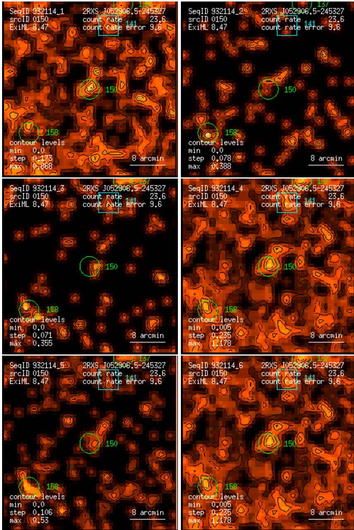
Figure 150: RASS 932114: detection 0150: band rate images, Gaussian filter: (1) PSPC channels 11 – 41, (2) 52 – 90, (3) 91 – 201, (4) 11 – 235, (5) 52 – 201, (6) 11 – 201. Broad band rates in counts/ks. Band rate contour levels in counts/ks/arcmin 2 .
