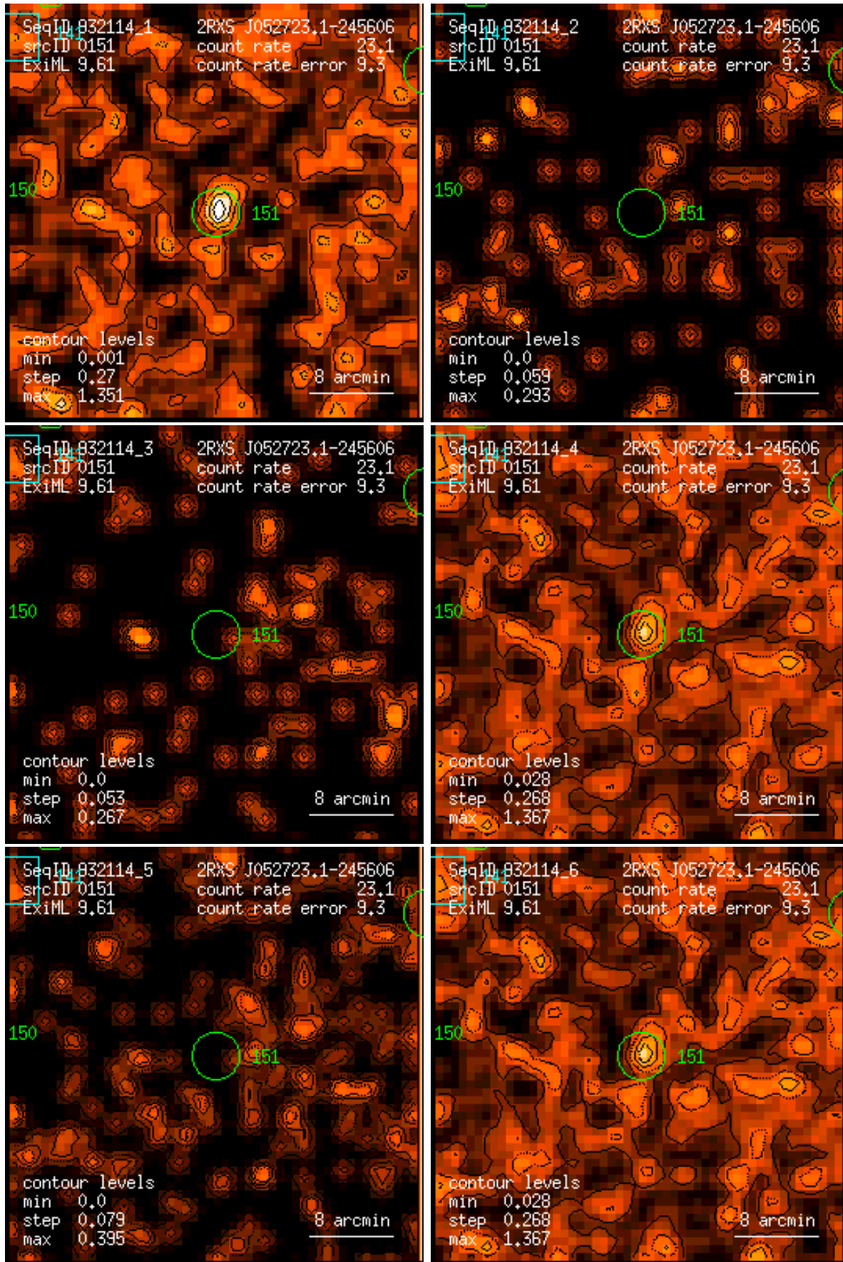
Figure 151: RASS 932114: detection 0151: band rate images, Gaussian filter: (1) PSPC channels 11 – 41, (2) 52 – 90, (3) 91 – 201, (4) 11 – 235, (5) 52 – 201, (6) 11 – 201. Broad band rates in counts/ks. Band rate contour levels in counts/ks/arcmin 2 .
