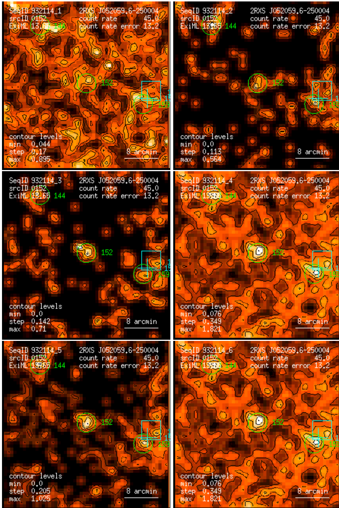
Figure 152: RASS 932114: detection 0152: band rate images, Gaussian filter: (1) PSPC channels 11 – 41, (2) 52 – 90, (3) 91 – 201, (4) 11 – 235, (5) 52 – 201, (6) 11 – 201. Broad band rates in counts/ks. Band rate contour levels in counts/ks/arcmin 2 .
