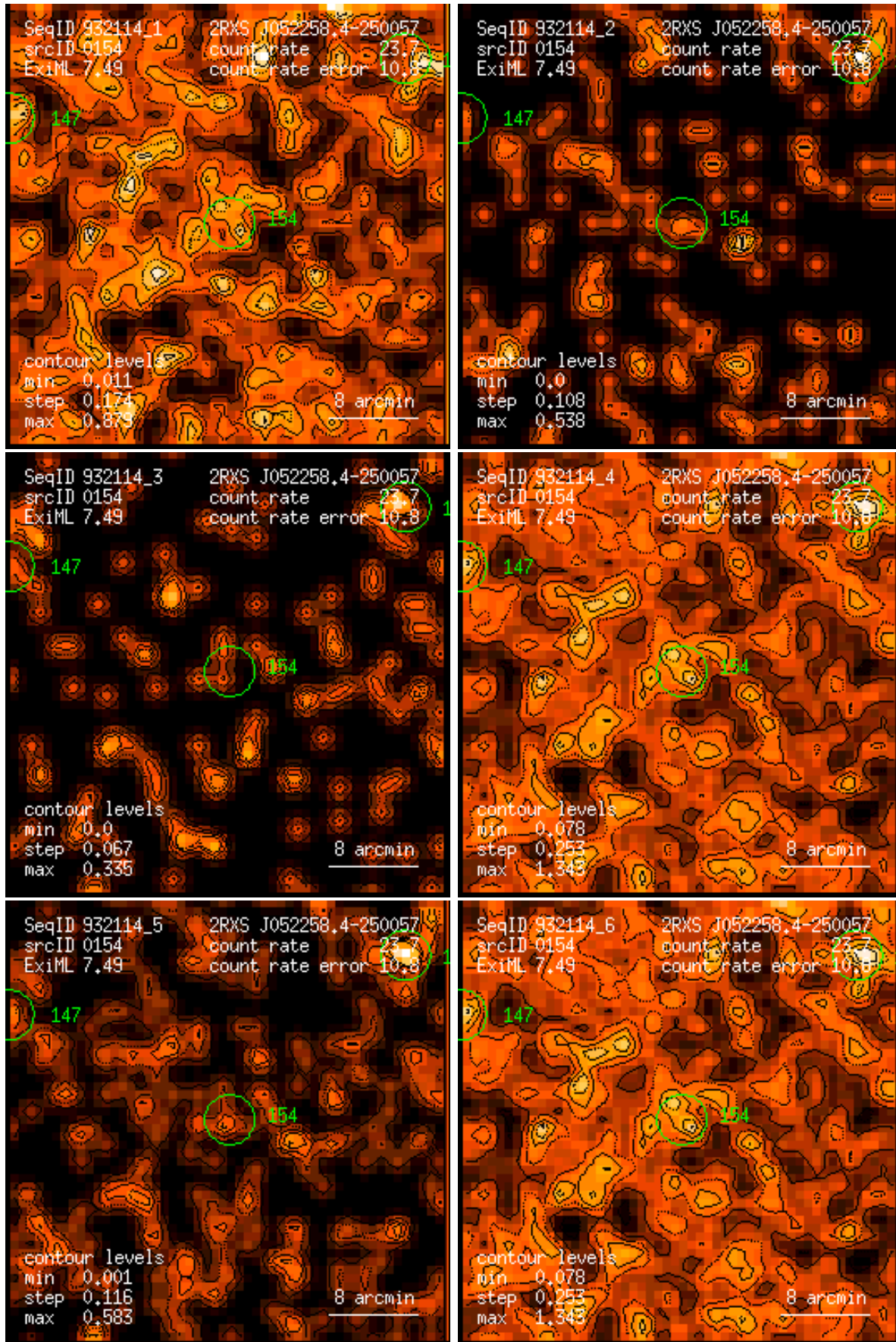
Figure 154: RASS 932114: detection 0154: band rate images, Gaussian filter: (1) PSPC channels 11 – 41, (2) 52 – 90, (3) 91 – 201, (4) 11 – 235, (5) 52 – 201, (6) 11 – 201. Broad band rates in counts/ks. Band rate contour levels in counts/ks/arcmin 2 .
