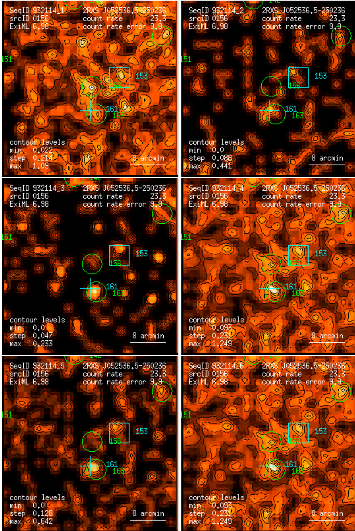
Figure 156: RASS 932114: detection 0156: band rate images, Gaussian filter: (1) PSPC channels 11 – 41, (2) 52 – 90, (3) 91 – 201, (4) 11 – 235, (5) 52 – 201, (6) 11 – 201. Broad band rates in counts/ks. Band rate contour levels in counts/ks/arcmin 2 .
