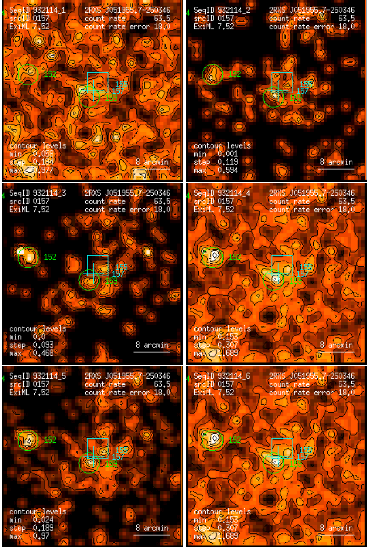
Figure 157: RASS 932114: detection 0157: band rate images, Gaussian filter: (1) PSPC channels 11 – 41, (2) 52 – 90, (3) 91 – 201, (4) 11 – 235, (5) 52 – 201, (6) 11 – 201. Broad band rates in counts/ks. Band rate contour levels in counts/ks/arcmin 2 .
