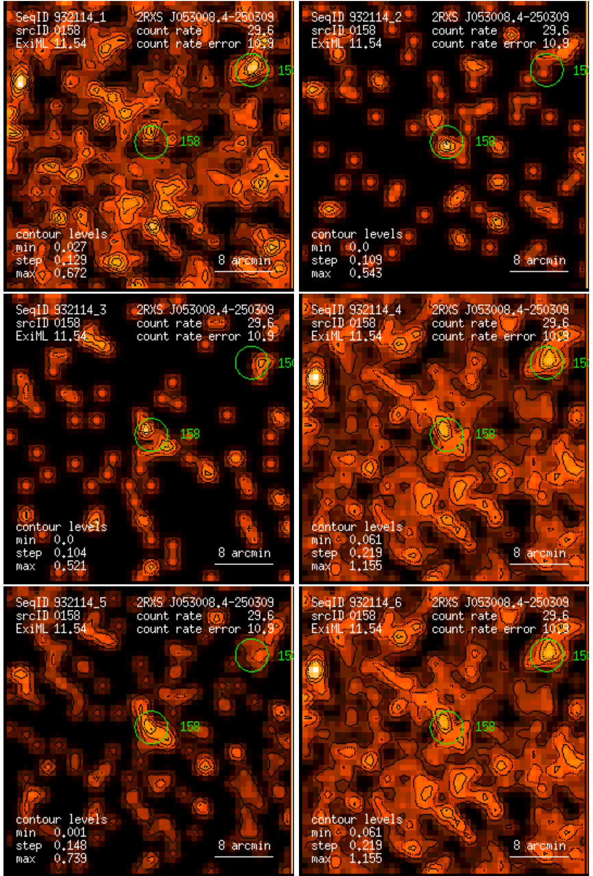
Figure 158: RASS 932114: detection 0158: band rate images, Gaussian filter: (1) PSPC channels 11 – 41, (2) 52 – 90, (3) 91 – 201, (4) 11 – 235, (5) 52 – 201, (6) 11 – 201. Broad band rates in counts/ks. Band rate contour levels in counts/ks/arcmin 2 .
