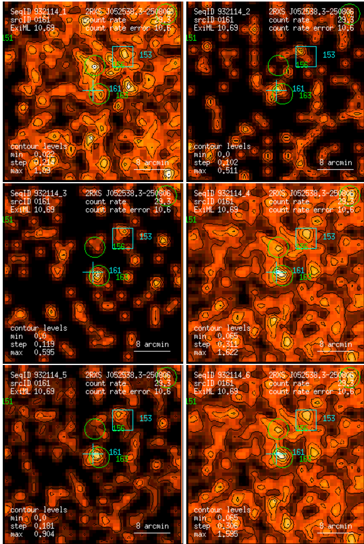
Figure 161: RASS 932114: detection 0161: band rate images, Gaussian filter: (1) PSPC channels 11 – 41, (2) 52 – 90, (3) 91 – 201, (4) 11 – 235, (5) 52 – 201, (6) 11 – 201. Broad band rates in counts/ks. Band rate contour levels in counts/ks/arcmin 2 .
