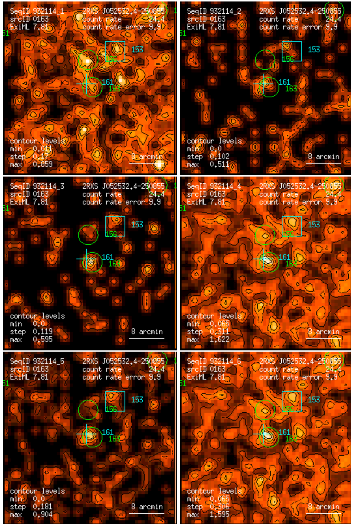
Figure 163: RASS 932114: detection 0163: band rate images, Gaussian filter: (1) PSPC channels 11 – 41, (2) 52 – 90, (3) 91 – 201, (4) 11 – 235, (5) 52 – 201, (6) 11 – 201. Broad band rates in counts/ks. Band rate contour levels in counts/ks/arcmin 2 .
