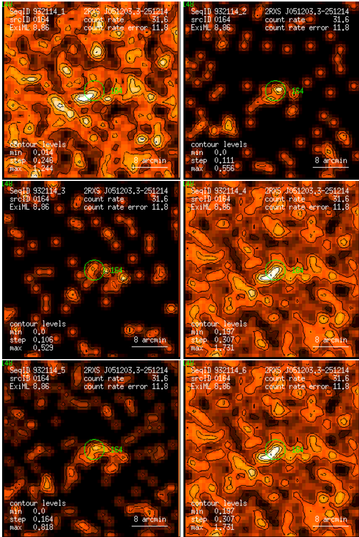
Figure 164: RASS 932114: detection 0164: band rate images, Gaussian filter: (1) PSPC channels 11 – 41, (2) 52 – 90, (3) 91 – 201, (4) 11 – 235, (5) 52 – 201, (6) 11 – 201. Broad band rates in counts/ks. Band rate contour levels in counts/ks/arcmin 2 .
