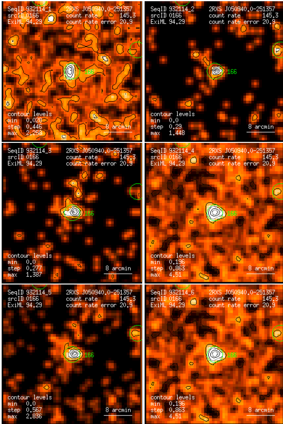
Figure 166: RASS 932114: detection 0166: band rate images, Gaussian filter: (1) PSPC channels 11 – 41, (2) 52 – 90, (3) 91 – 201, (4) 11 – 235, (5) 52 – 201, (6) 11 – 201. Broad band rates in counts/ks. Band rate contour levels in counts/ks/arcmin 2 .
