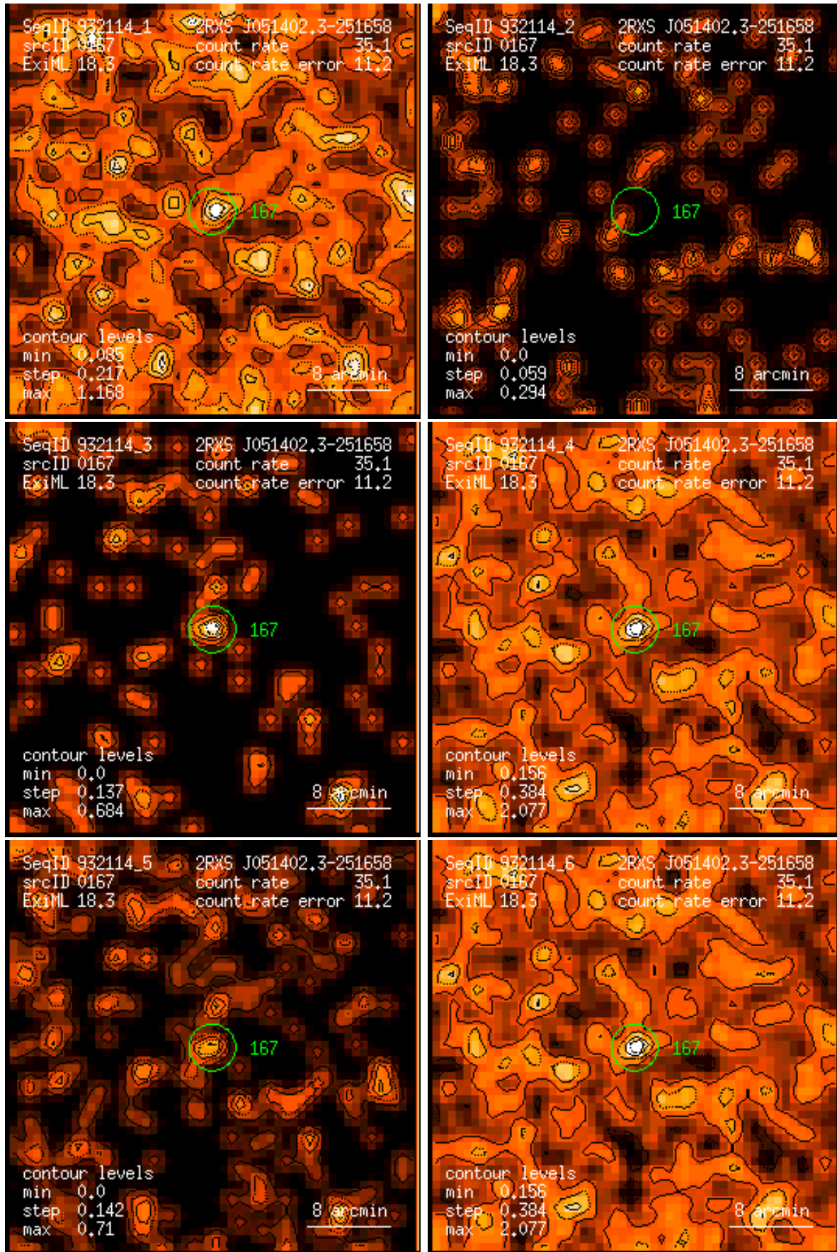
Figure 167: RASS 932114: detection 0167: band rate images, Gaussian filter: (1) PSPC channels 11 – 41, (2) 52 – 90, (3) 91 – 201, (4) 11 – 235, (5) 52 – 201, (6) 11 – 201. Broad band rates in counts/ks. Band rate contour levels in counts/ks/arcmin 2 .
