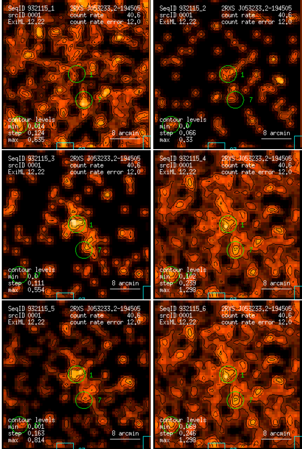
Figure 1: RASS 932115: detection 0001: band rate images, Gaussian filter: (1) PSPC channels 11 – 41, (2) 52 – 90, (3) 91 – 201, (4) 11 – 235, (5) 52 – 201, (6) 11 – 201. Broad band rates in counts/ks. Band rate contour levels in counts/ks/arcmin 2 .
