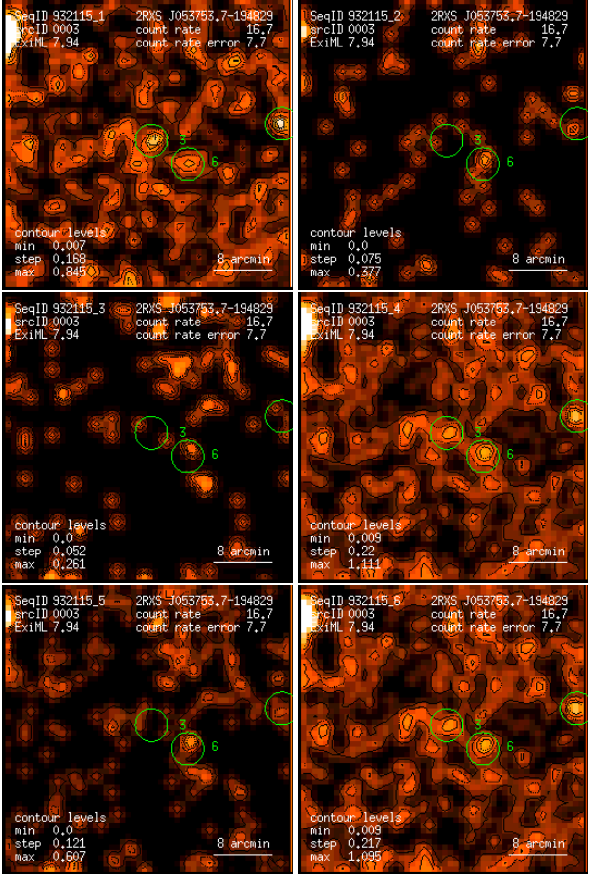
Figure 3: RASS 932115: detection 0003: band rate images, Gaussian filter: (1) PSPC channels 11 – 41, (2) 52 – 90, (3) 91 – 201, (4) 11 – 235, (5) 52 – 201, (6) 11 – 201. Broad band rates in counts/ks. Band rate contour levels in counts/ks/arcmin 2 .
