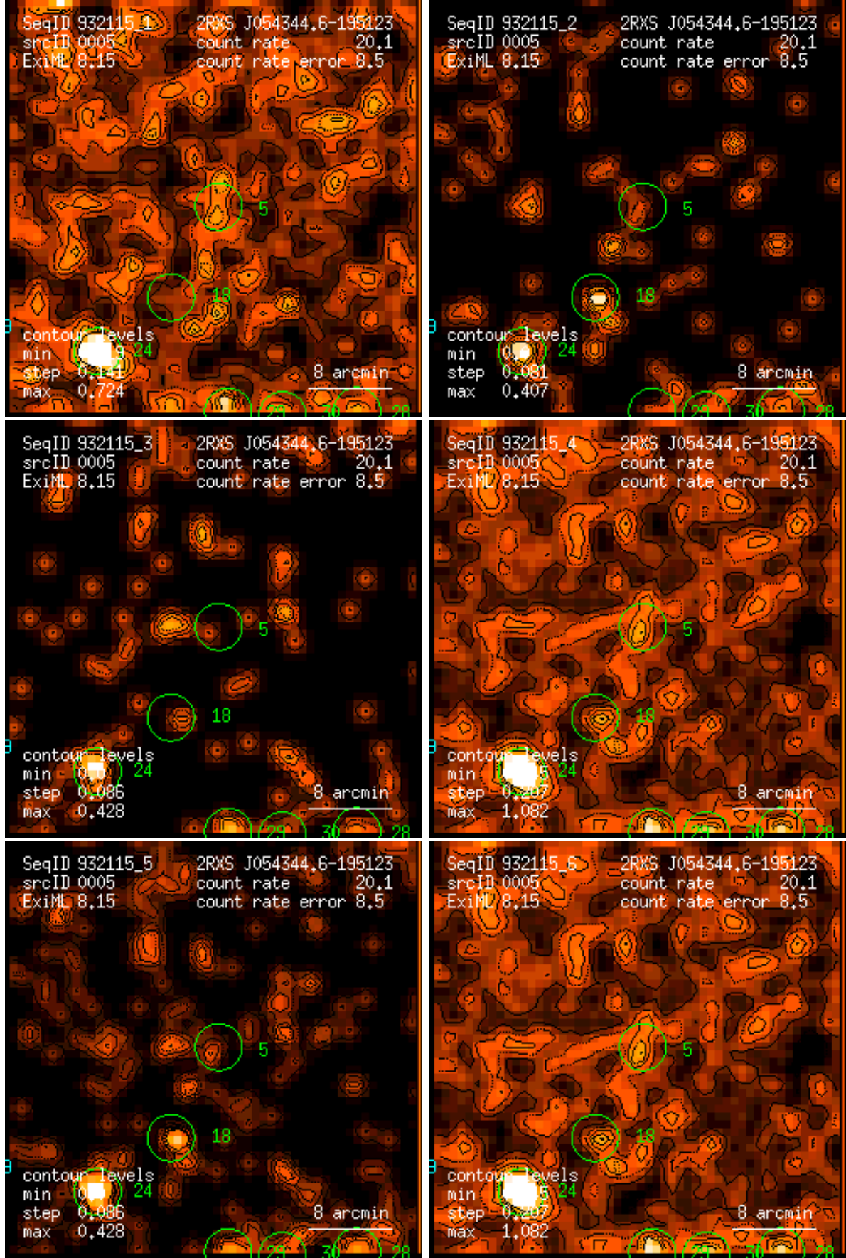
Figure 5: RASS 932115: detection 0005: band rate images, Gaussian filter: (1) PSPC channels 11 – 41, (2) 52 – 90, (3) 91 – 201, (4) 11 – 235, (5) 52 – 201, (6) 11 – 201. Broad band rates in counts/ks. Band rate contour levels in counts/ks/arcmin 2 .
