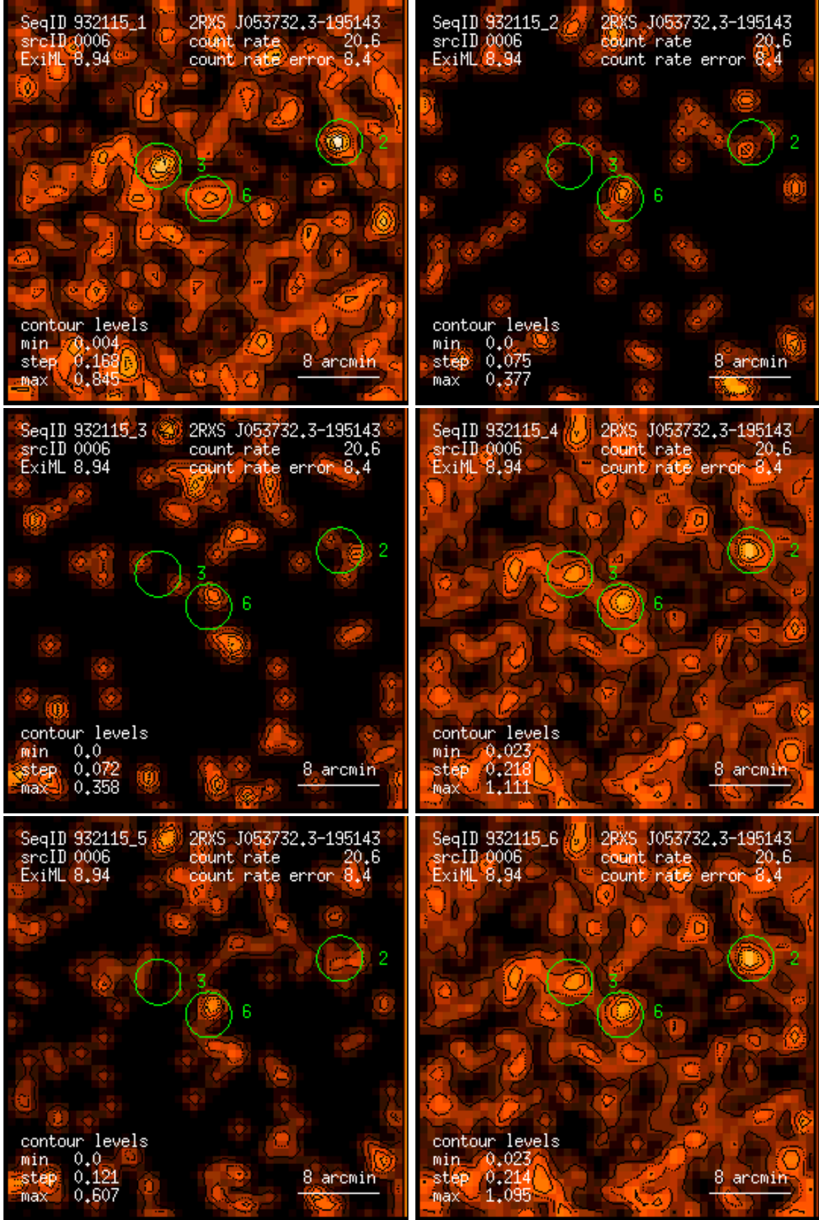
Figure 6: RASS 932115: detection 0006: band rate images, Gaussian filter: (1) PSPC channels 11 – 41, (2) 52 – 90, (3) 91 – 201, (4) 11 – 235, (5) 52 – 201, (6) 11 – 201. Broad band rates in counts/ks. Band rate contour levels in counts/ks/arcmin 2 .
