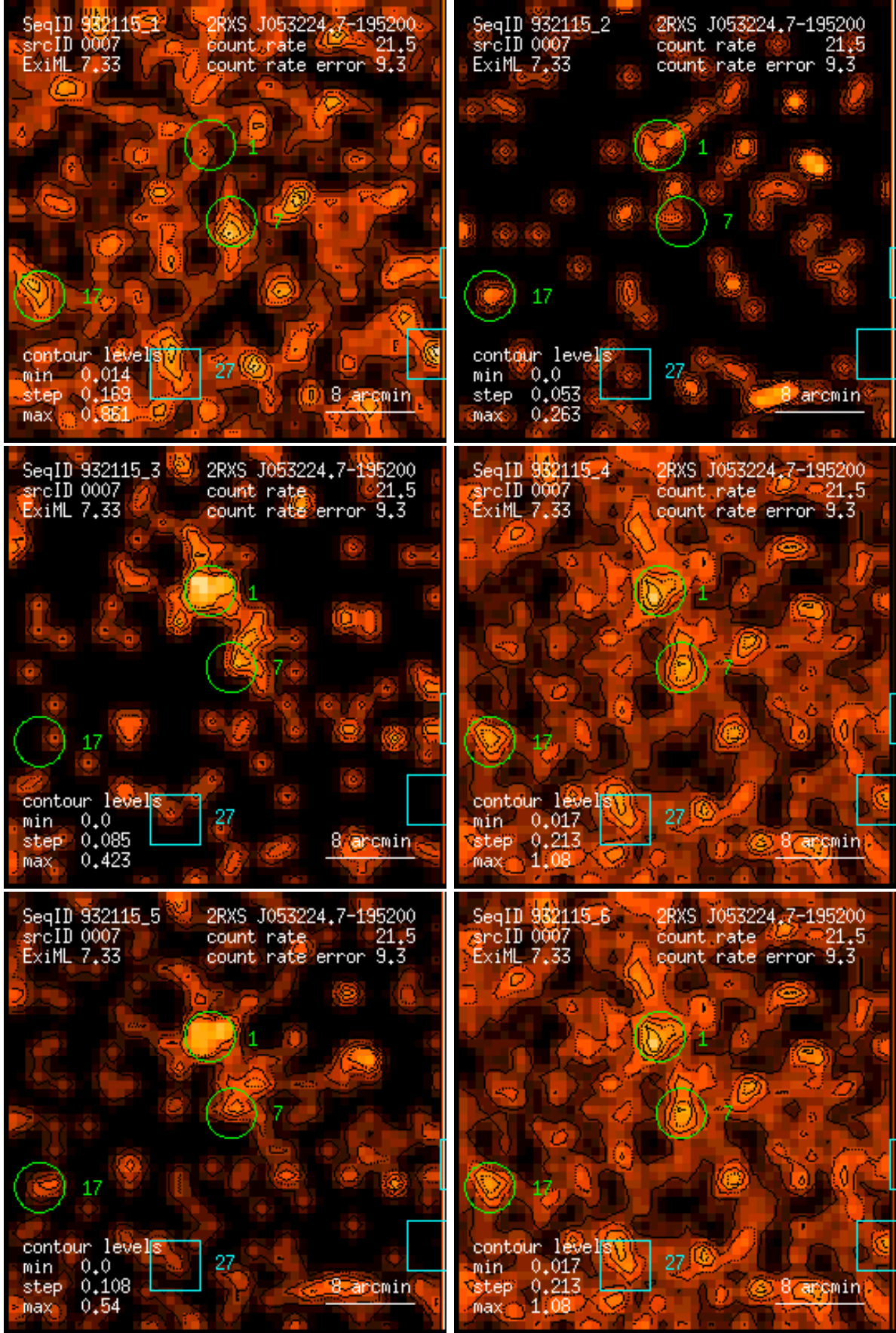
Figure 7: RASS 932115: detection 0007: band rate images, Gaussian filter: (1) PSPC channels 11 – 41, (2) 52 – 90, (3) 91 – 201, (4) 11 – 235, (5) 52 – 201, (6) 11 – 201. Broad band rates in counts/ks. Band rate contour levels in counts/ks/arcmin 2 .
