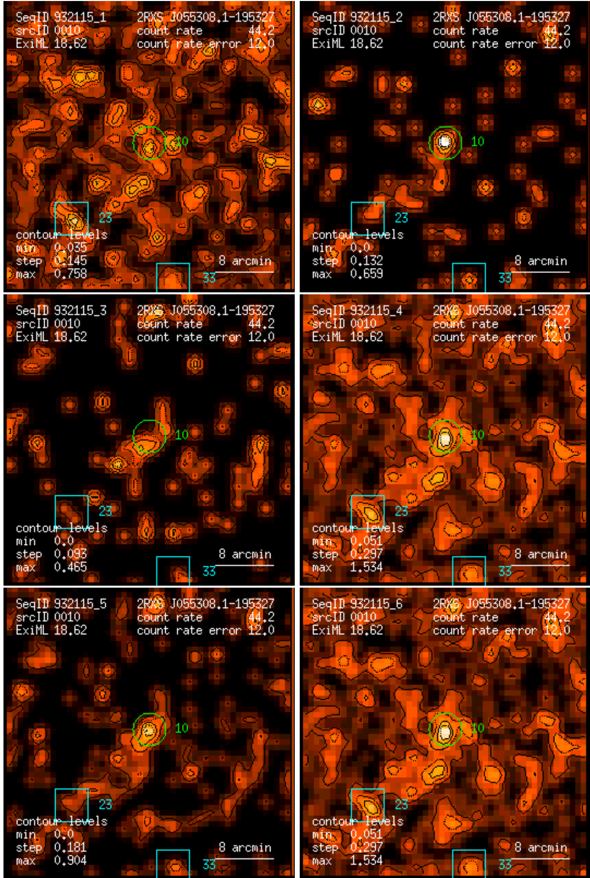
Figure 10: RASS 932115: detection 0010: band rate images, Gaussian filter: (1) PSPC channels 11 – 41, (2) 52 – 90, (3) 91 – 201, (4) 11 – 235, (5) 52 – 201, (6) 11 – 201. Broad band rates in counts/ks. Band rate contour levels in counts/ks/arcmin 2 .
