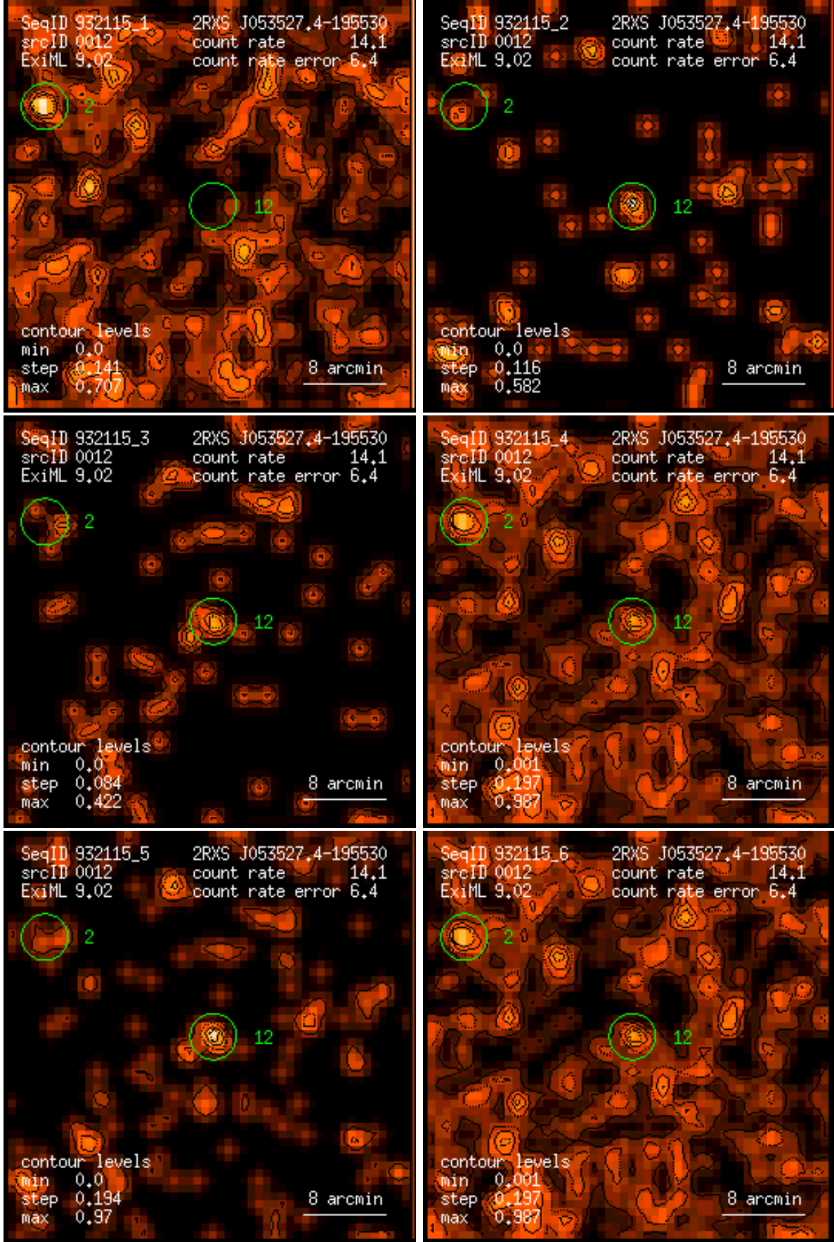
Figure 12: RASS 932115: detection 0012: band rate images, Gaussian filter: (1) PSPC channels 11 – 41, (2) 52 – 90, (3) 91 – 201, (4) 11 – 235, (5) 52 – 201, (6) 11 – 201. Broad band rates in counts/ks. Band rate contour levels in counts/ks/arcmin 2 .
