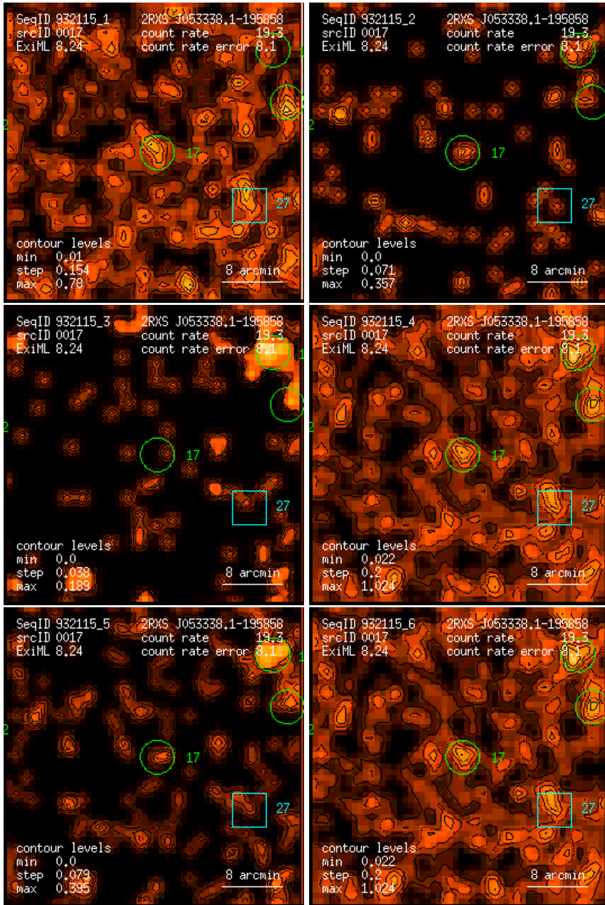
Figure 17: RASS 932115: detection 0017: band rate images, Gaussian filter: (1) PSPC channels 11 – 41, (2) 52 – 90, (3) 91 – 201, (4) 11 – 235, (5) 52 – 201, (6) 11 – 201. Broad band rates in counts/ks. Band rate contour levels in counts/ks/arcmin 2 .
