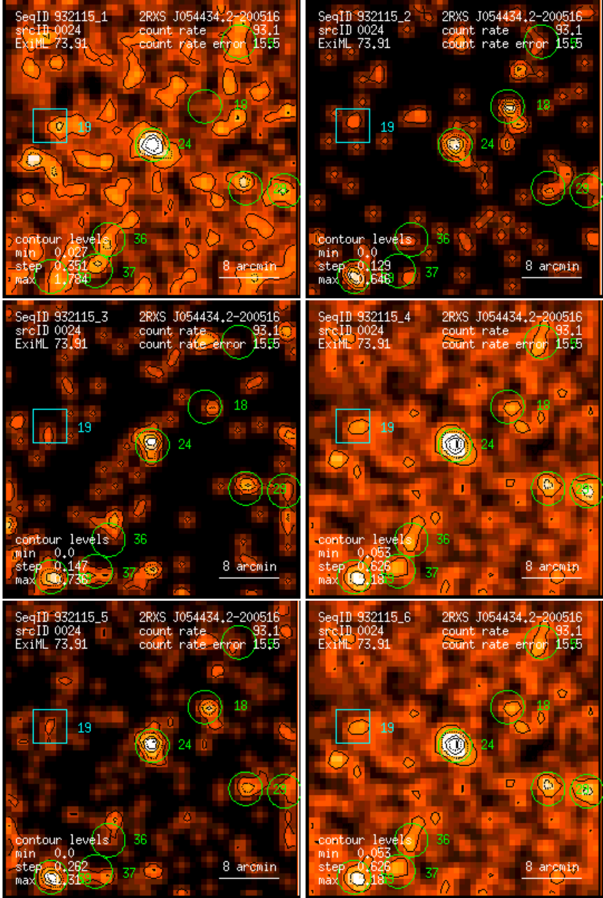
Figure 24: RASS 932115: detection 0024: band rate images, Gaussian filter: (1) PSPC channels 11 – 41, (2) 52 – 90, (3) 91 – 201, (4) 11 – 235, (5) 52 – 201, (6) 11 – 201. Broad band rates in counts/ks. Band rate contour levels in counts/ks/arcmin 2 .
