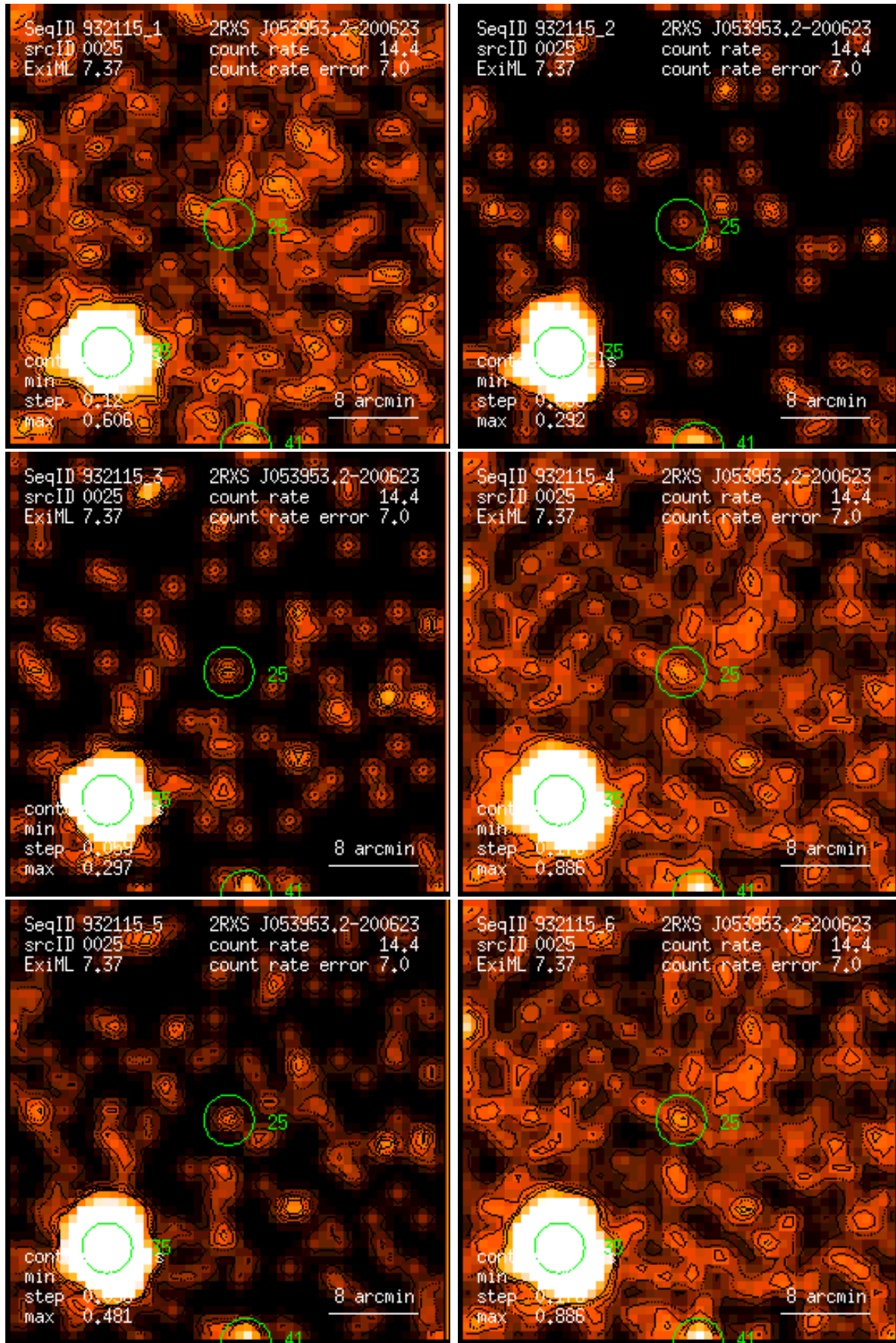
Figure 25: RASS 932115: detection 0025: band rate images, Gaussian filter: (1) PSPC channels 11 – 41, (2) 52 – 90, (3) 91 – 201, (4) 11 – 235, (5) 52 – 201, (6) 11 – 201. Broad band rates in counts/ks. Band rate contour levels in counts/ks/arcmin 2 .
