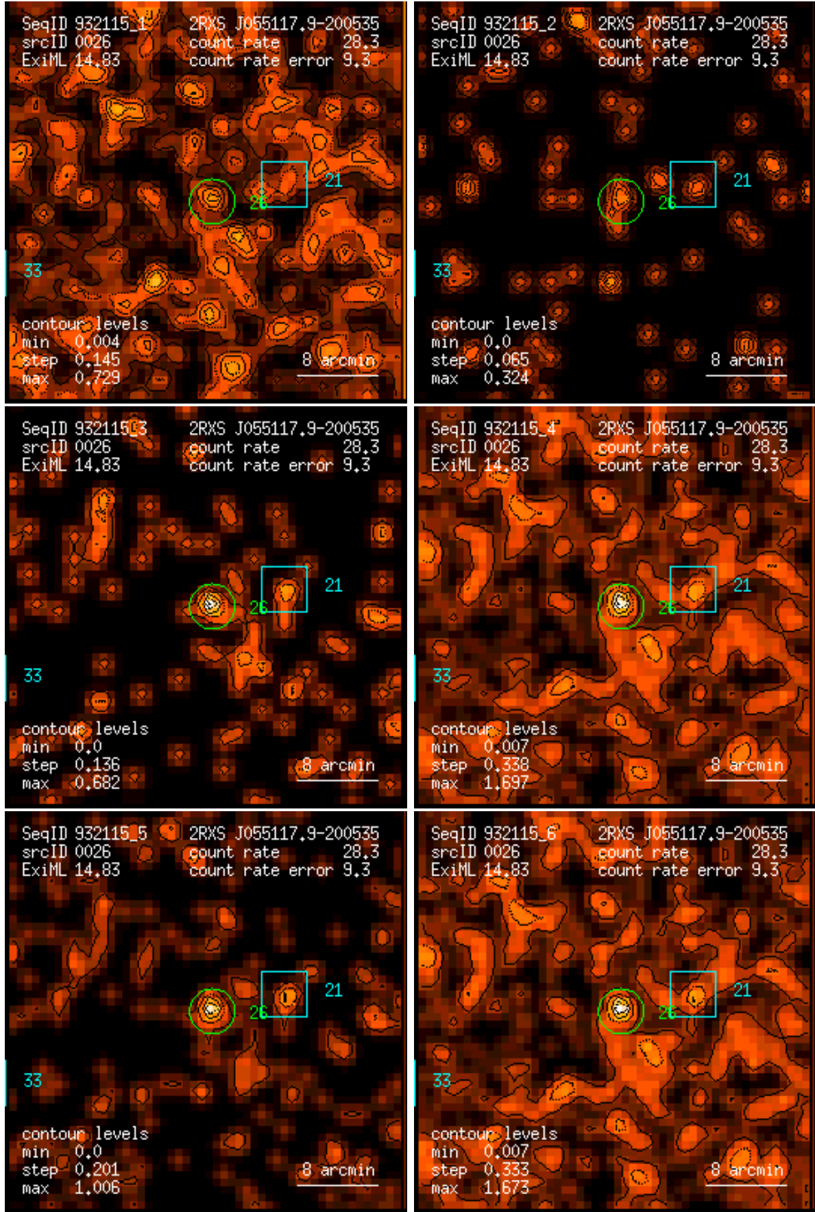
Figure 26: RASS 932115: detection 0026: band rate images, Gaussian filter: (1) PSPC channels 11 – 41, (2) 52 – 90, (3) 91 – 201, (4) 11 – 235, (5) 52 – 201, (6) 11 – 201. Broad band rates in counts/ks. Band rate contour levels in counts/ks/arcmin 2 .
