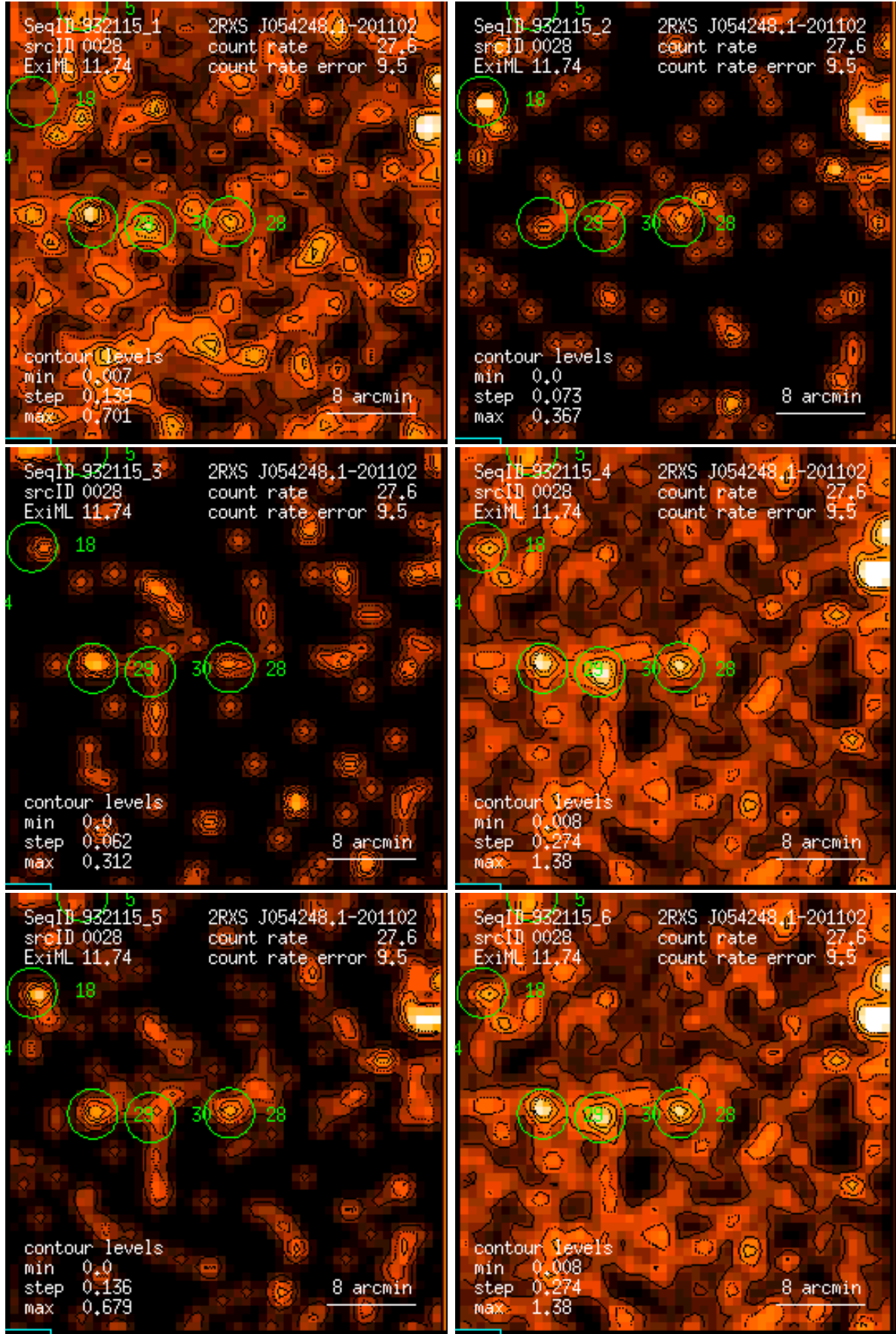
Figure 28: RASS 932115: detection 0028: band rate images, Gaussian filter: (1) PSPC channels 11 – 41, (2) 52 – 90, (3) 91 – 201, (4) 11 – 235, (5) 52 – 201, (6) 11 – 201. Broad band rates in counts/ks. Band rate contour levels in counts/ks/arcmin 2 .
