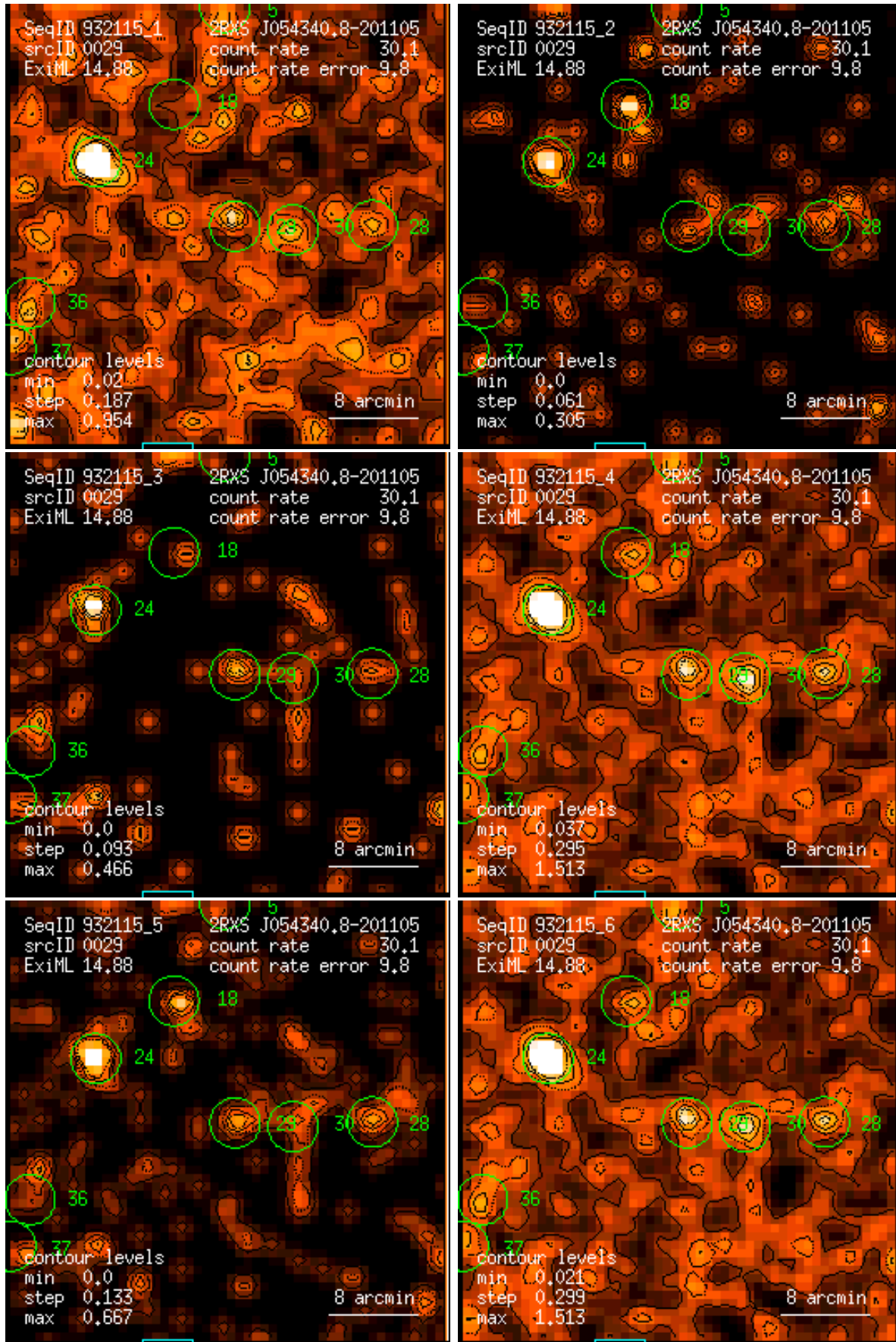
Figure 29: RASS 932115: detection 0029: band rate images, Gaussian filter: (1) PSPC channels 11 – 41, (2) 52 – 90, (3) 91 – 201, (4) 11 – 235, (5) 52 – 201, (6) 11 – 201. Broad band rates in counts/ks. Band rate contour levels in counts/ks/arcmin 2 .
