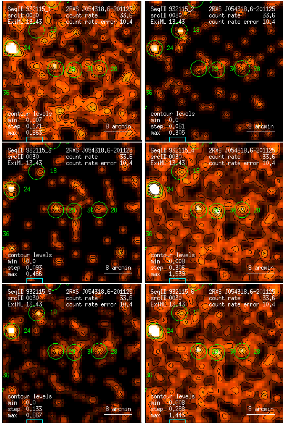
Figure 30: RASS 932115: detection 0030: band rate images, Gaussian filter: (1) PSPC channels 11 – 41, (2) 52 – 90, (3) 91 – 201, (4) 11 – 235, (5) 52 – 201, (6) 11 – 201. Broad band rates in counts/ks. Band rate contour levels in counts/ks/arcmin 2 .
