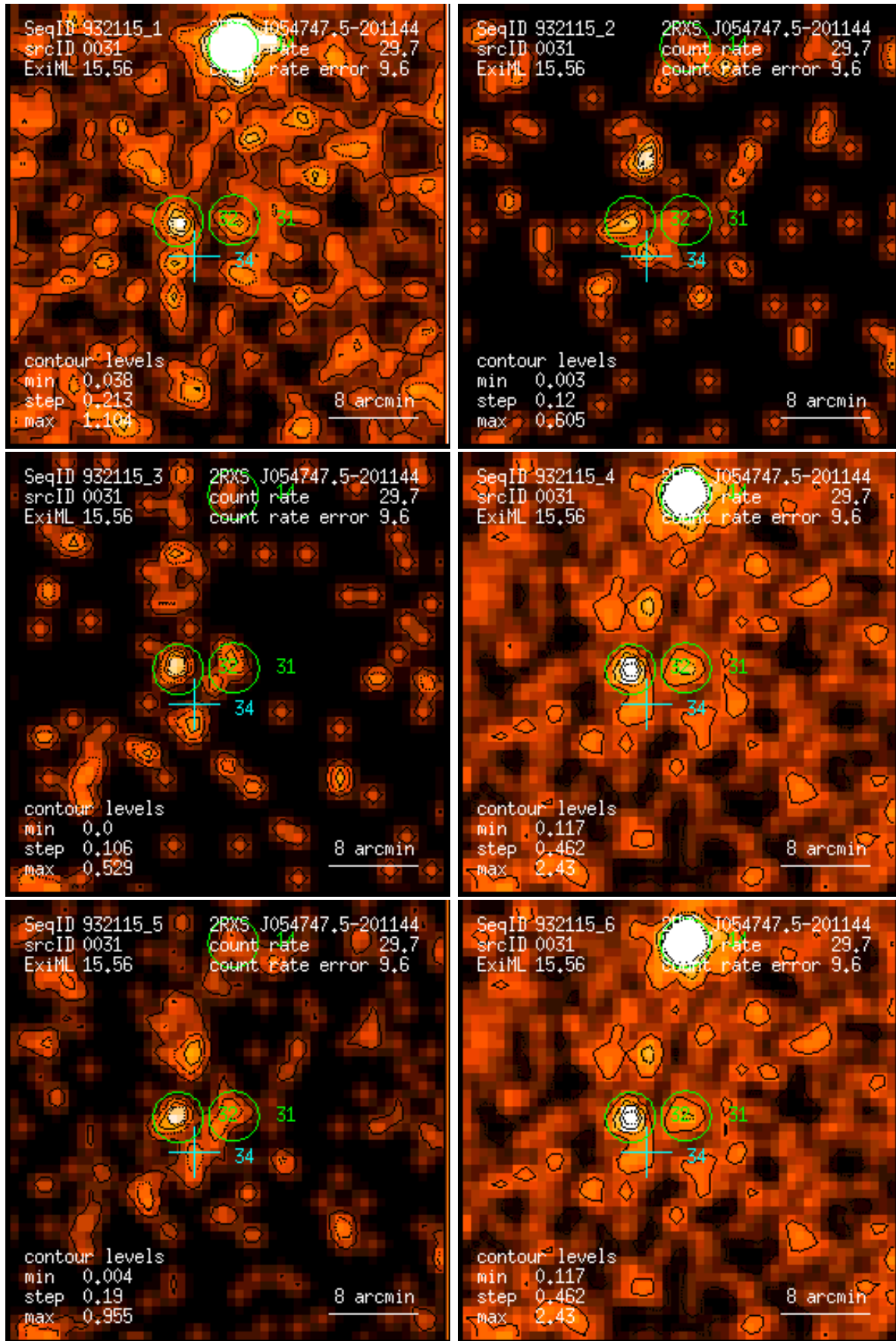
Figure 31: RASS 932115: detection 0031: band rate images, Gaussian filter: (1) PSPC channels 11 – 41, (2) 52 – 90, (3) 91 – 201, (4) 11 – 235, (5) 52 – 201, (6) 11 – 201. Broad band rates in counts/ks. Band rate contour levels in counts/ks/arcmin 2 .
