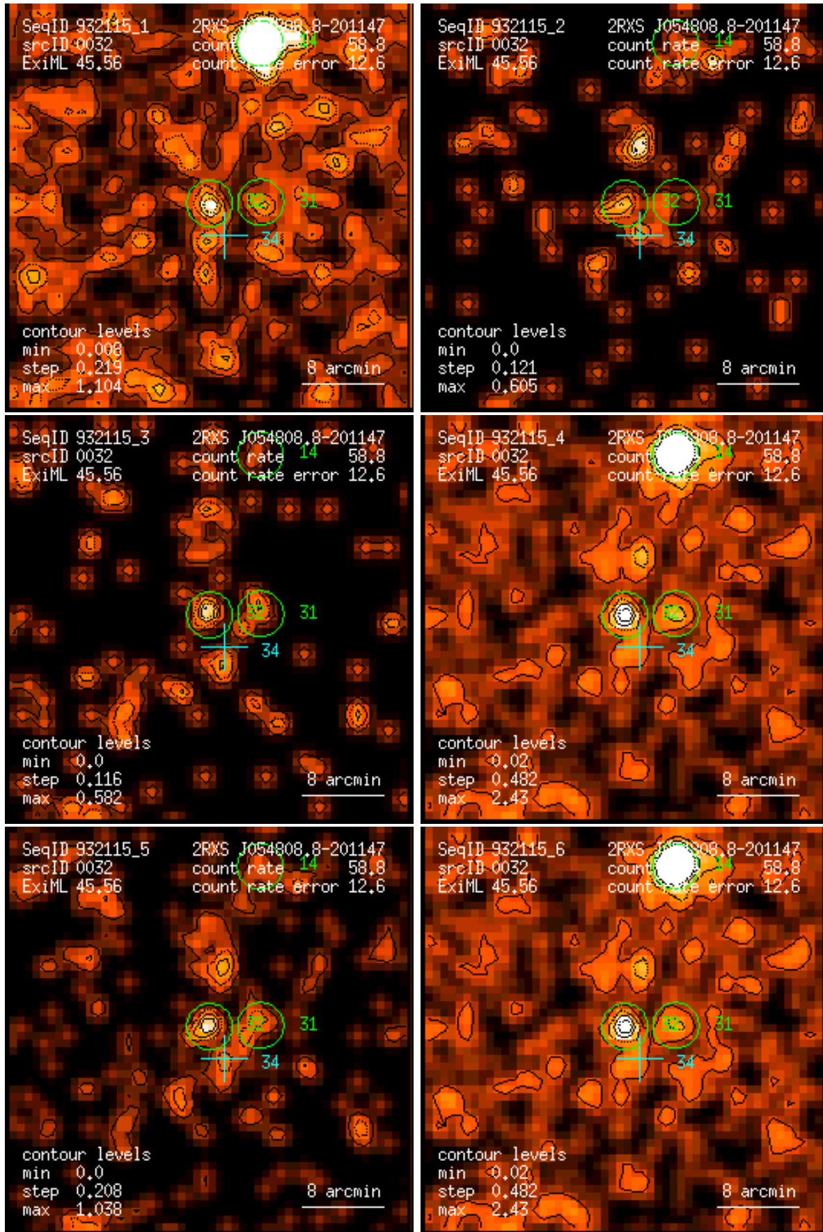
Figure 32: RASS 932115: detection 0032: band rate images, Gaussian filter: (1) PSPC channels 11 – 41, (2) 52 – 90, (3) 91 – 201, (4) 11 – 235, (5) 52 – 201, (6) 11 – 201. Broad band rates in counts/ks. Band rate contour levels in counts/ks/arcmin 2 .
