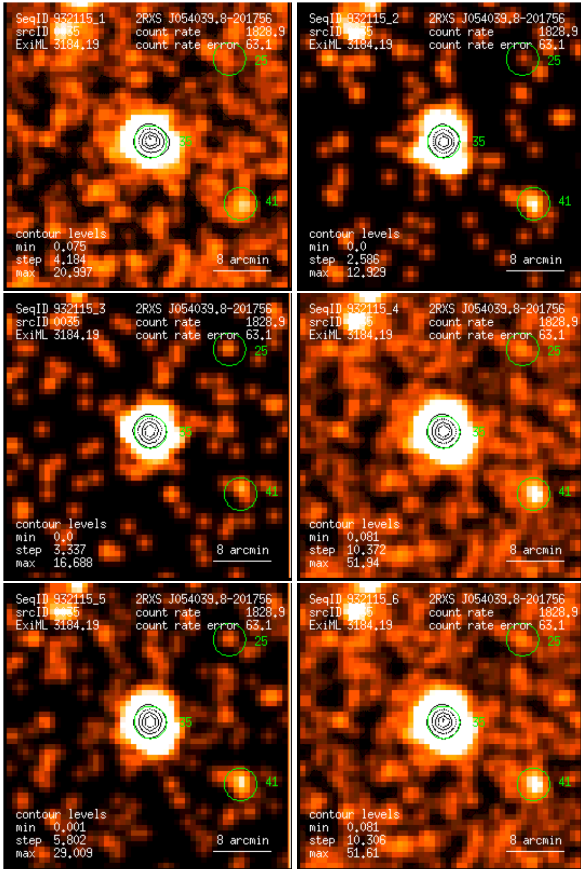
Figure 35: RASS 932115: detection 0035: band rate images, Gaussian filter: (1) PSPC channels 11 – 41, (2) 52 – 90, (3) 91 – 201, (4) 11 – 235, (5) 52 – 201, (6) 11 – 201. Broad band rates in counts/ks. Band rate contour levels in counts/ks/arcmin 2 .
