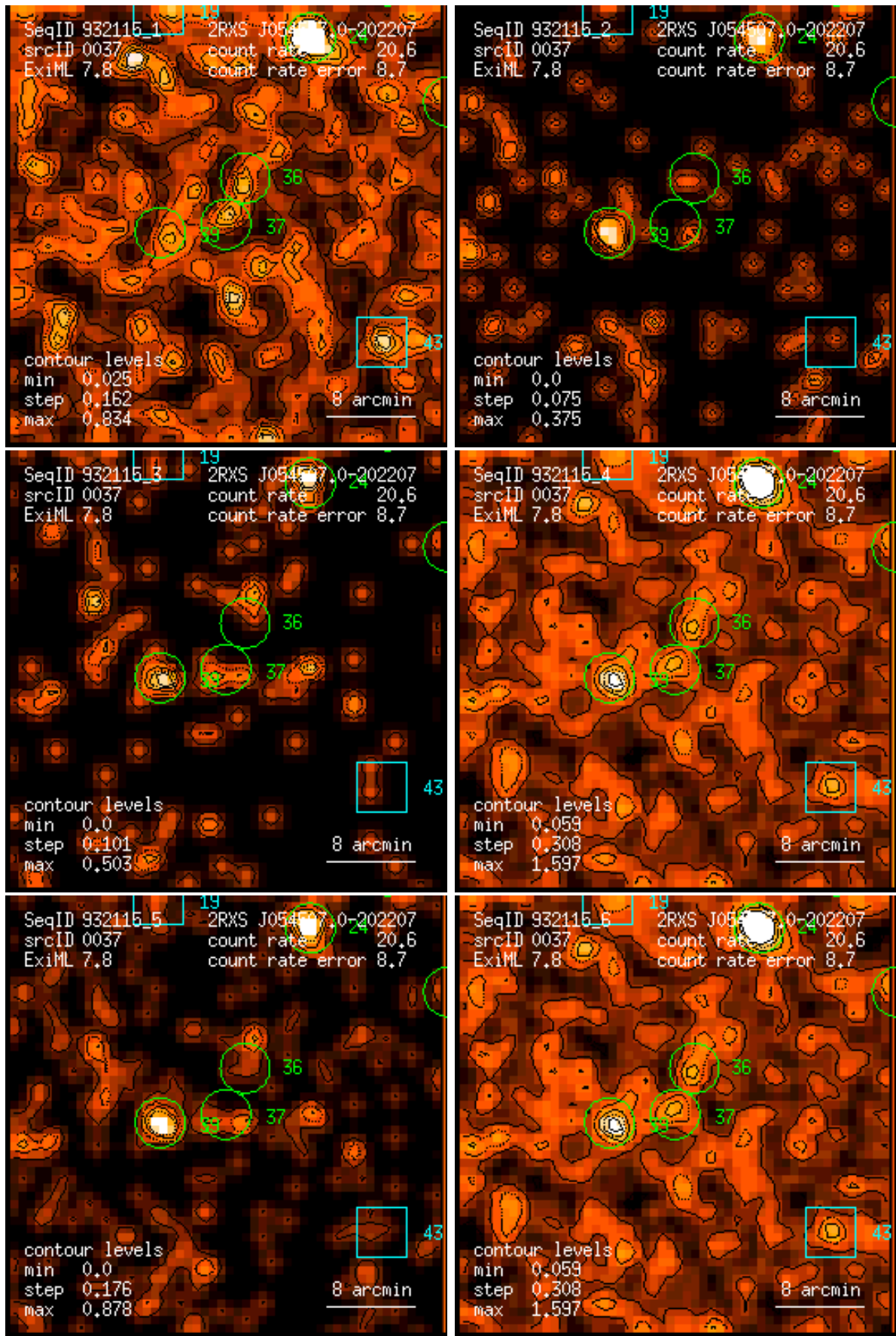
Figure 37: RASS 932115: detection 0037: band rate images, Gaussian filter: (1) PSPC channels 11 – 41, (2) 52 – 90, (3) 91 – 201, (4) 11 – 235, (5) 52 – 201, (6) 11 – 201. Broad band rates in counts/ks. Band rate contour levels in counts/ks/arcmin 2 .
