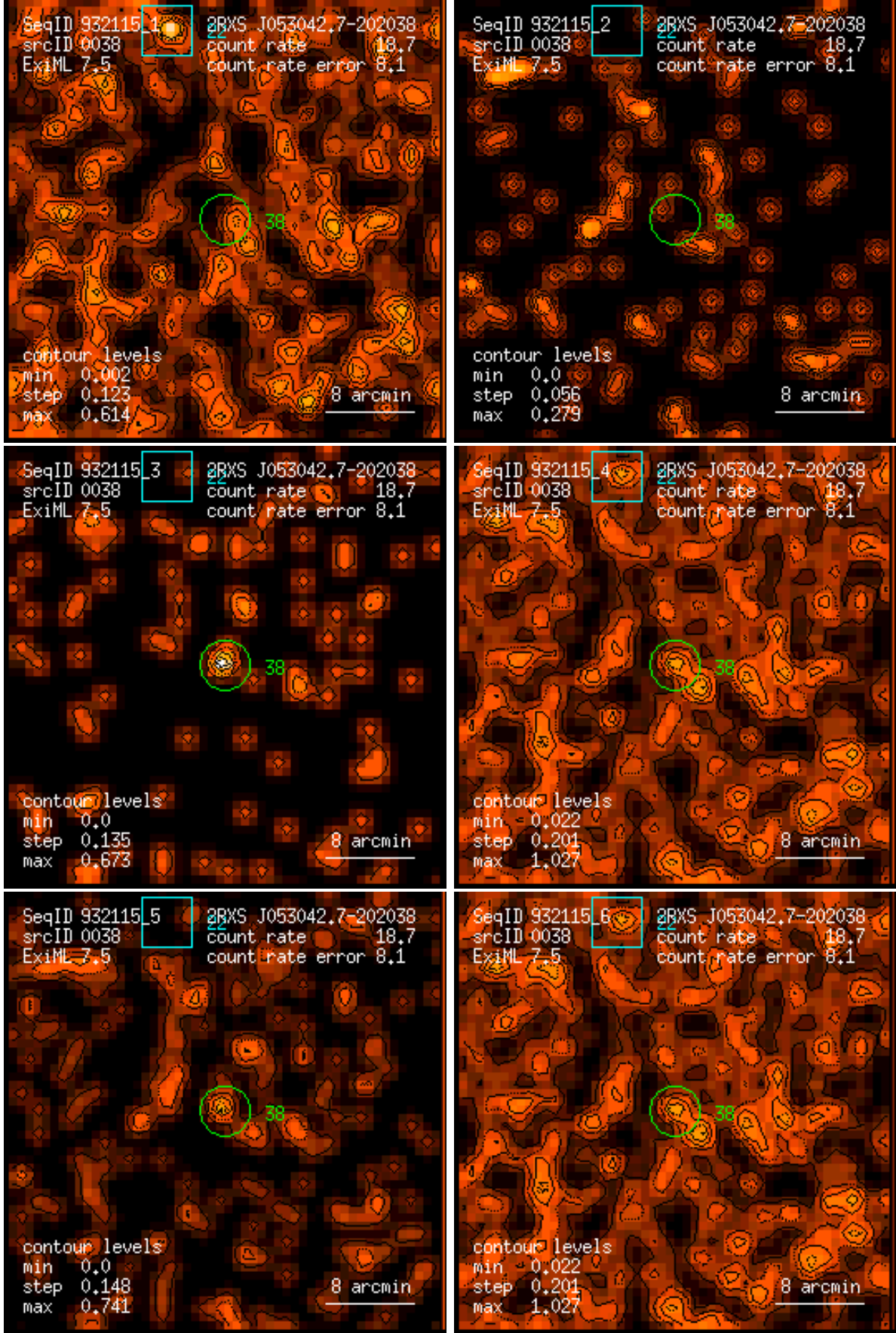
Figure 38: RASS 932115: detection 0038: band rate images, Gaussian filter: (1) PSPC channels 11 – 41, (2) 52 – 90, (3) 91 – 201, (4) 11 – 235, (5) 52 – 201, (6) 11 – 201. Broad band rates in counts/ks. Band rate contour levels in counts/ks/arcmin 2 .
