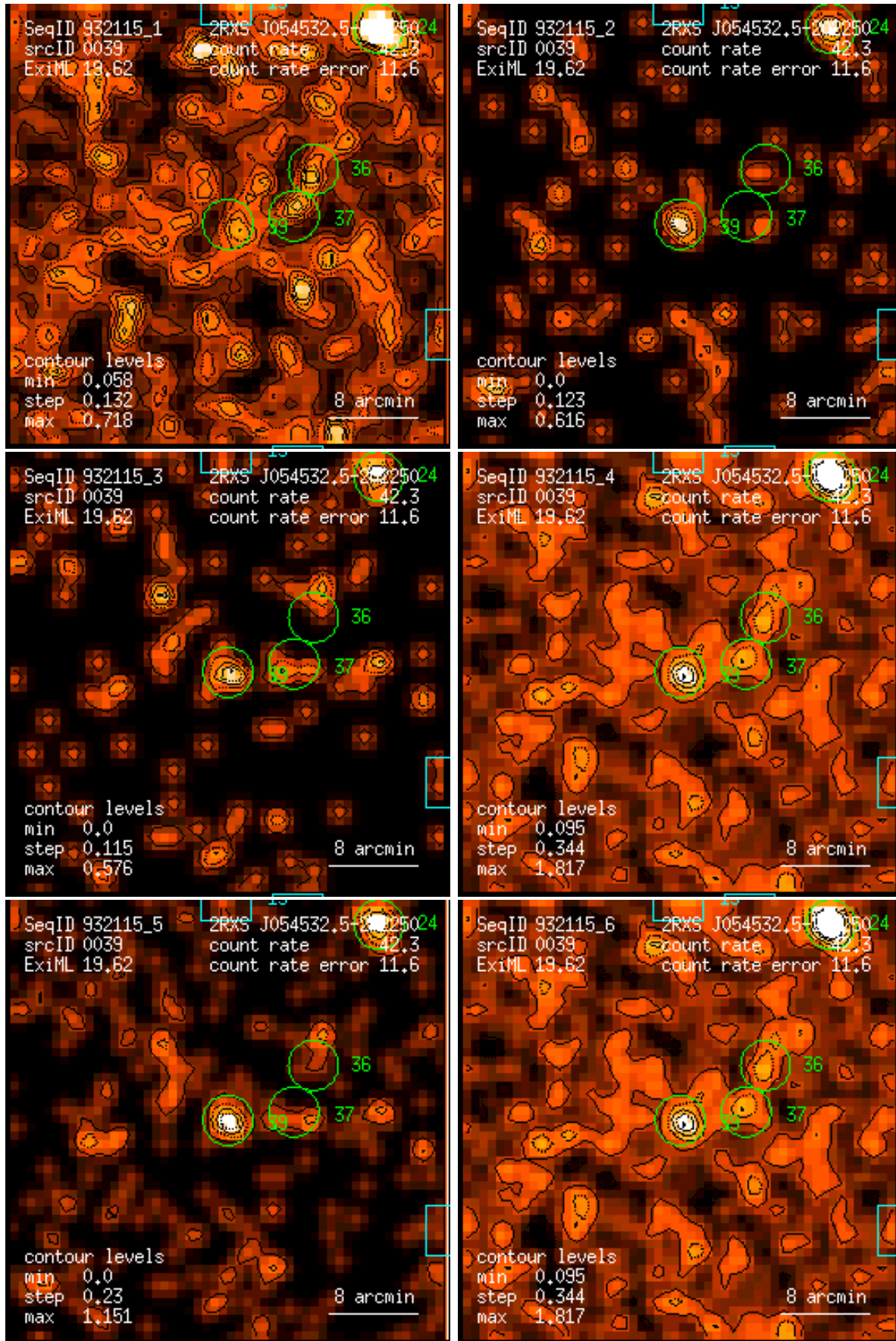
Figure 39: RASS 932115: detection 0039: band rate images, Gaussian filter: (1) PSPC channels 11 – 41, (2) 52 – 90, (3) 91 – 201, (4) 11 – 235, (5) 52 – 201, (6) 11 – 201. Broad band rates in counts/ks. Band rate contour levels in counts/ks/arcmin 2 .
