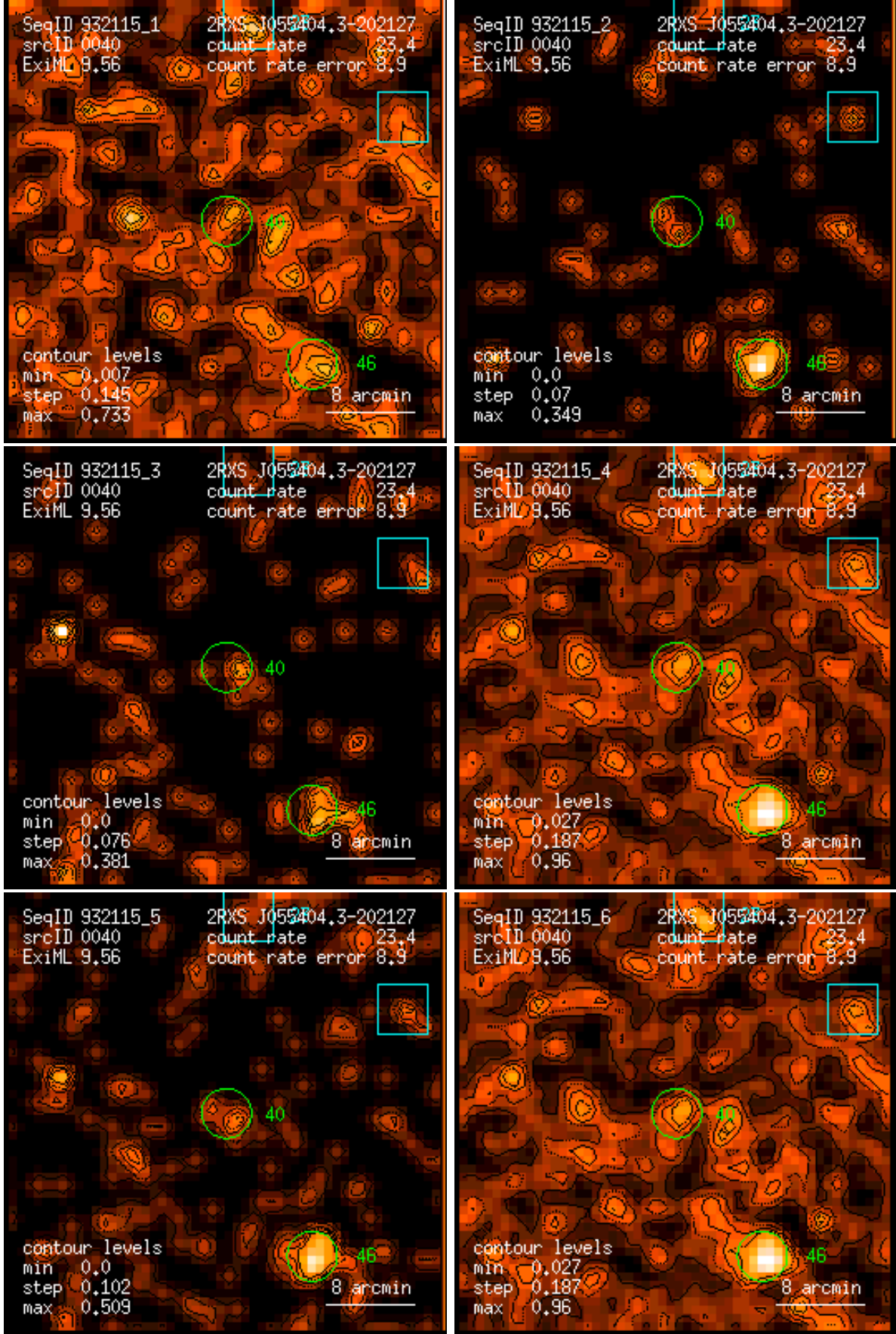
Figure 40: RASS 932115: detection 0040: band rate images, Gaussian filter: (1) PSPC channels 11 – 41, (2) 52 – 90, (3) 91 – 201, (4) 11 – 235, (5) 52 – 201, (6) 11 – 201. Broad band rates in counts/ks. Band rate contour levels in counts/ks/arcmin 2 .
