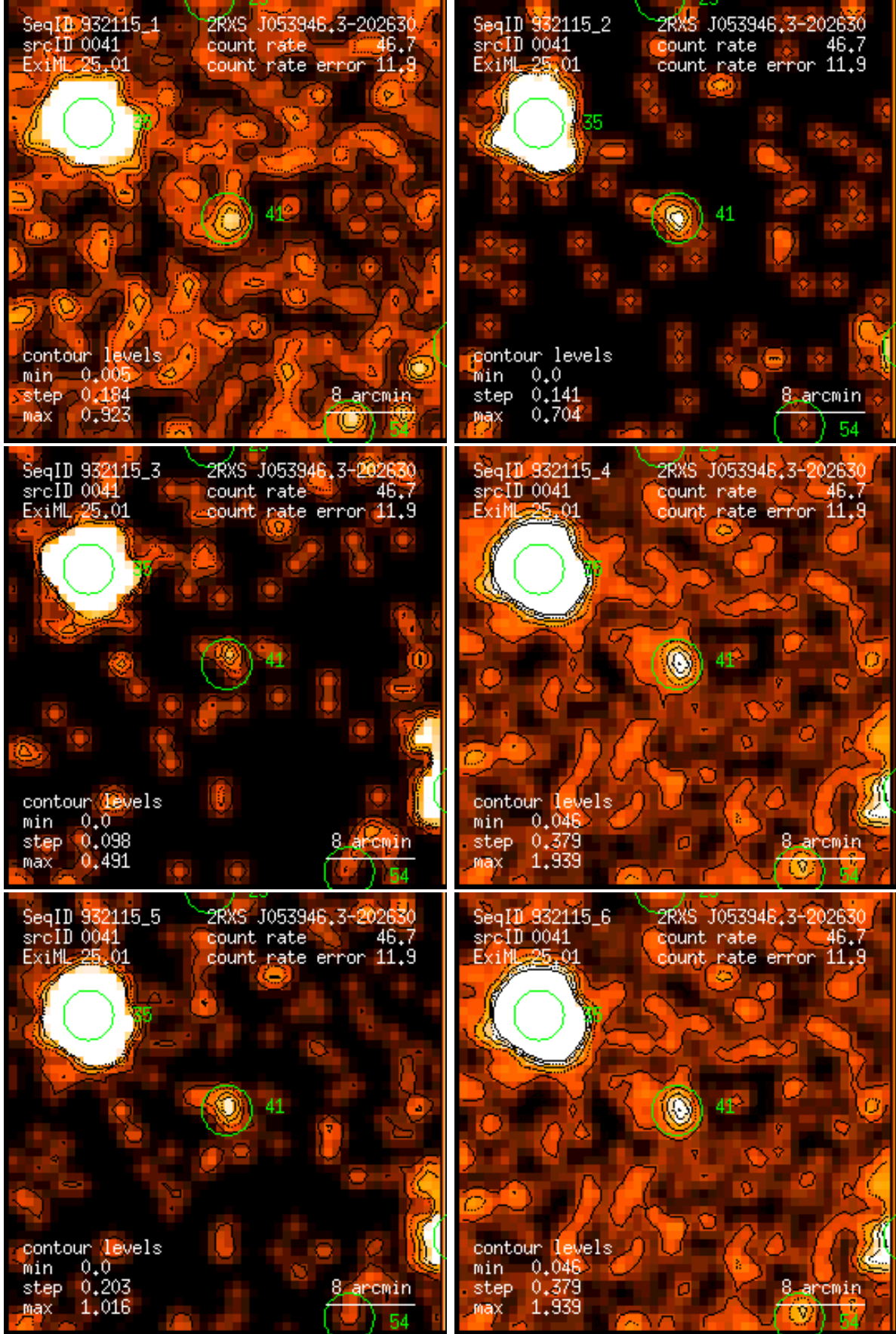
Figure 41: RASS 932115: detection 0041: band rate images, Gaussian filter: (1) PSPC channels 11 – 41, (2) 52 – 90, (3) 91 – 201, (4) 11 – 235, (5) 52 – 201, (6) 11 – 201. Broad band rates in counts/ks. Band rate contour levels in counts/ks/arcmin 2 .
