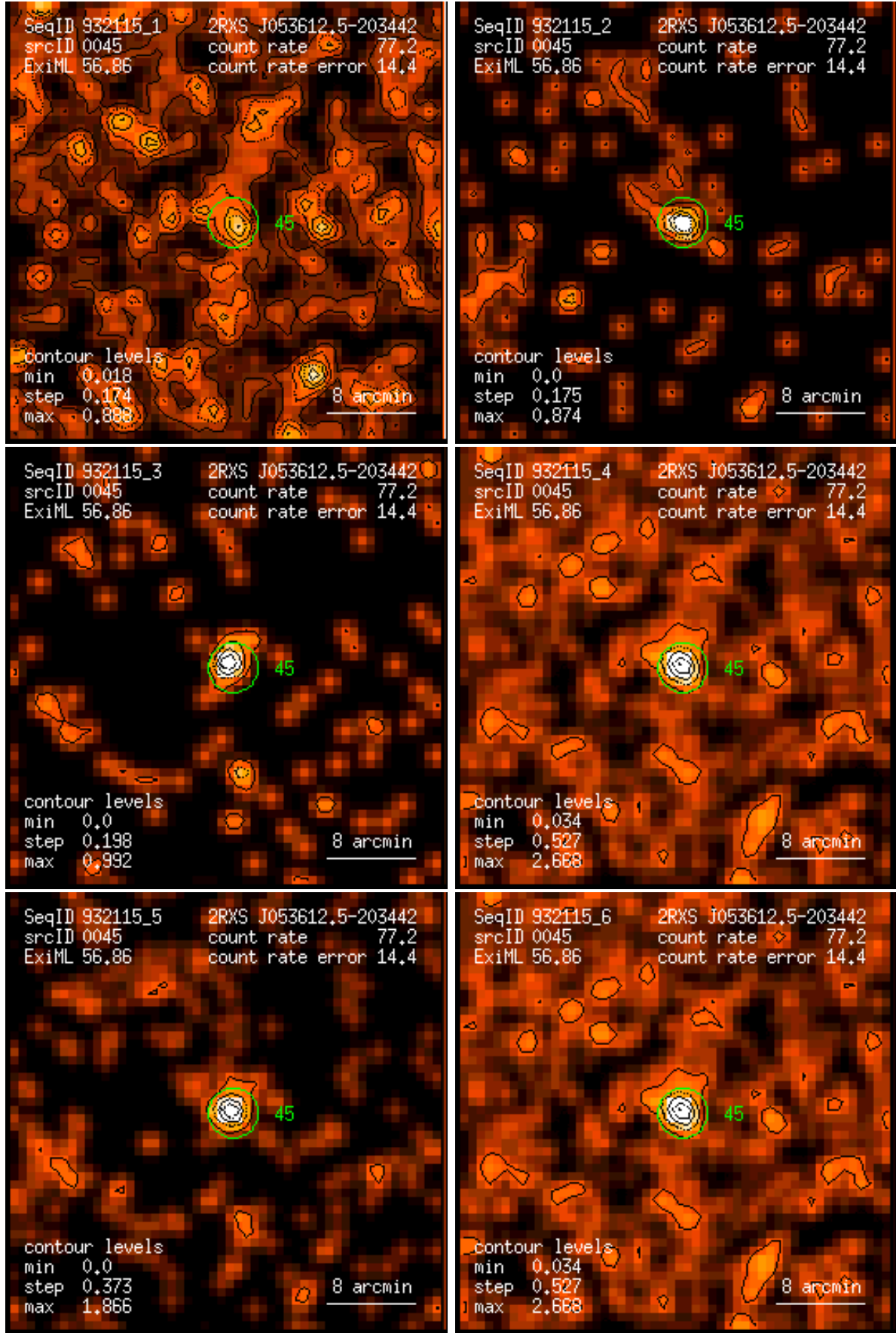
Figure 45: RASS 932115: detection 0045: band rate images, Gaussian filter: (1) PSPC channels 11 – 41, (2) 52 – 90, (3) 91 – 201, (4) 11 – 235, (5) 52 – 201, (6) 11 – 201. Broad band rates in counts/ks. Band rate contour levels in counts/ks/arcmin 2 .
