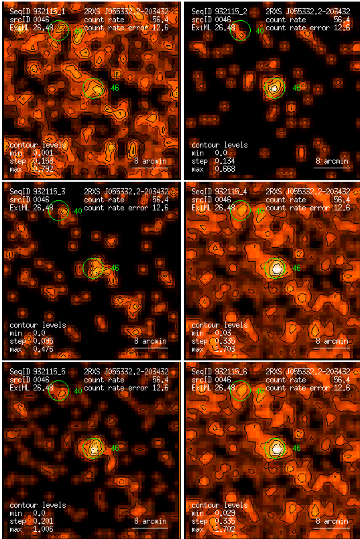
Figure 46: RASS 932115: detection 0046: band rate images, Gaussian filter: (1) PSPC channels 11 – 41, (2) 52 – 90, (3) 91 – 201, (4) 11 – 235, (5) 52 – 201, (6) 11 – 201. Broad band rates in counts/ks. Band rate contour levels in counts/ks/arcmin 2 .
