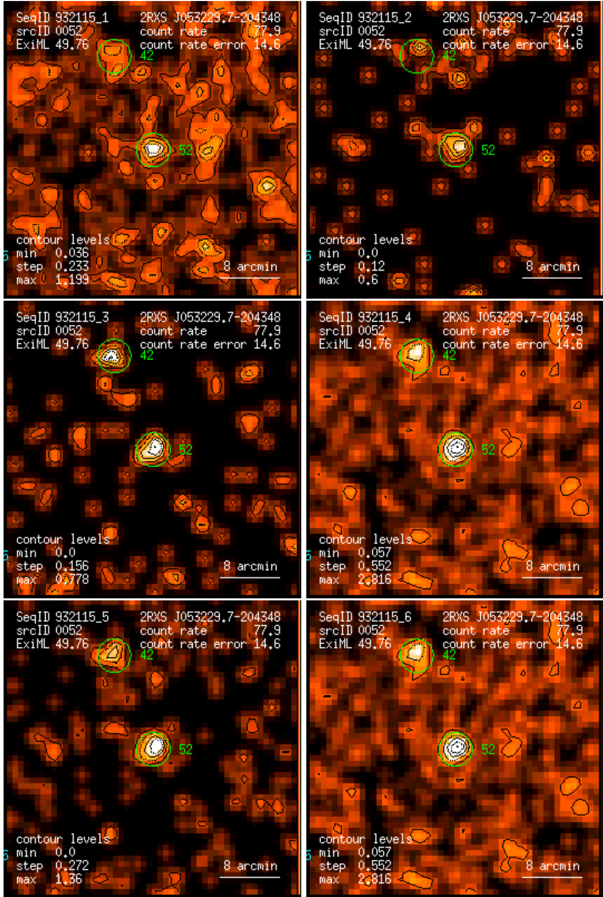
Figure 52: RASS 932115: detection 0052: band rate images, Gaussian filter: (1) PSPC channels 11 – 41, (2) 52 – 90, (3) 91 – 201, (4) 11 – 235, (5) 52 – 201, (6) 11 – 201. Broad band rates in counts/ks. Band rate contour levels in counts/ks/arcmin 2 .
