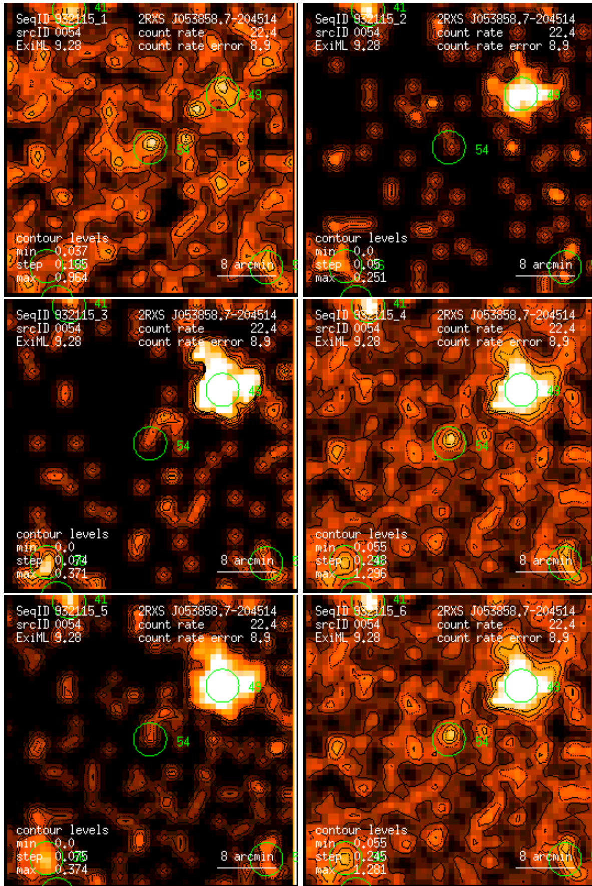
Figure 54: RASS 932115: detection 0054: band rate images, Gaussian filter: (1) PSPC channels 11 – 41, (2) 52 – 90, (3) 91 – 201, (4) 11 – 235, (5) 52 – 201, (6) 11 – 201. Broad band rates in counts/ks. Band rate contour levels in counts/ks/arcmin 2 .
