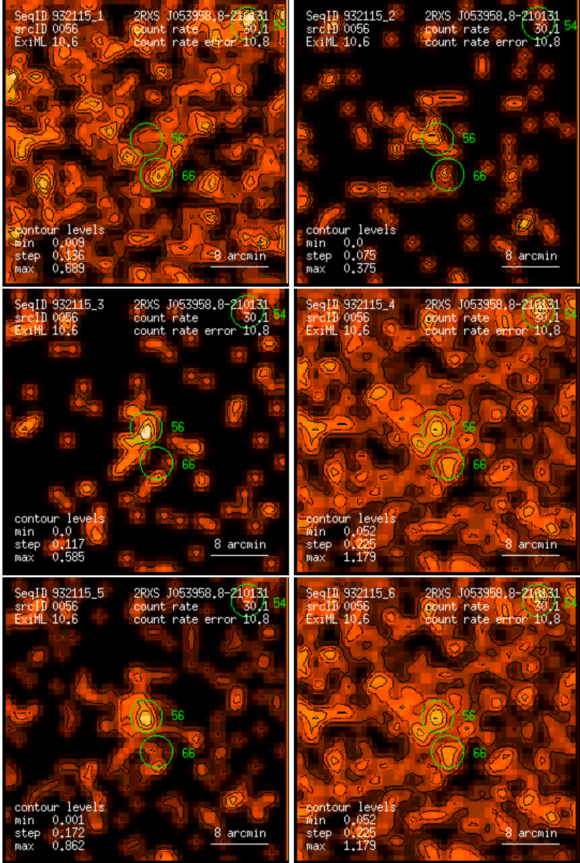
Figure 56: RASS 932115: detection 0056: band rate images, Gaussian filter: (1) PSPC channels 11 – 41, (2) 52 – 90, (3) 91 – 201, (4) 11 – 235, (5) 52 – 201, (6) 11 – 201. Broad band rates in counts/ks. Band rate contour levels in counts/ks/arcmin 2 .
