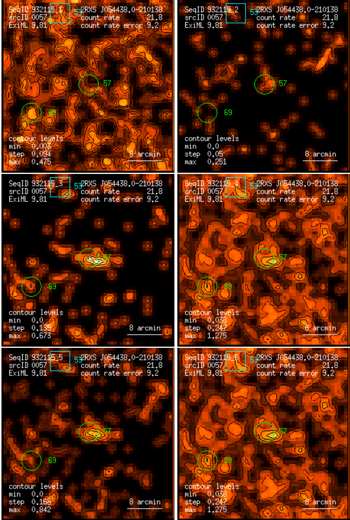
Figure 57: RASS 932115: detection 0057: band rate images, Gaussian filter: (1) PSPC channels 11 – 41, (2) 52 – 90, (3) 91 – 201, (4) 11 – 235, (5) 52 – 201, (6) 11 – 201. Broad band rates in counts/ks. Band rate contour levels in counts/ks/arcmin 2 .
